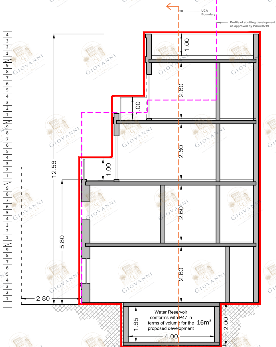
Longitudinal Section X : X PROPOSED Scale 1:100
