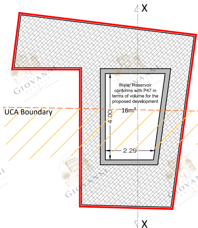
BASEMENT LEVEL PROPOSED Scale 1:100
