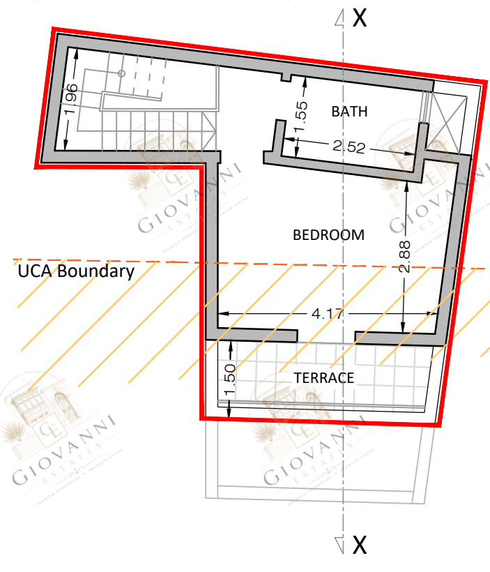
RECEDED FLOOR PROPOSED Scale 1:100
