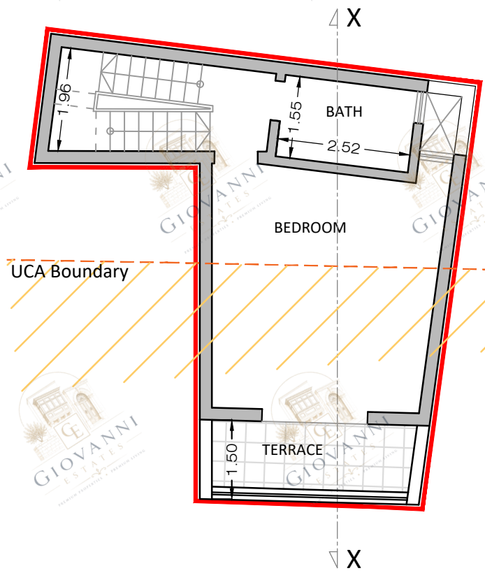
SECOND FLOOR PROPOSED Scale 1:100
