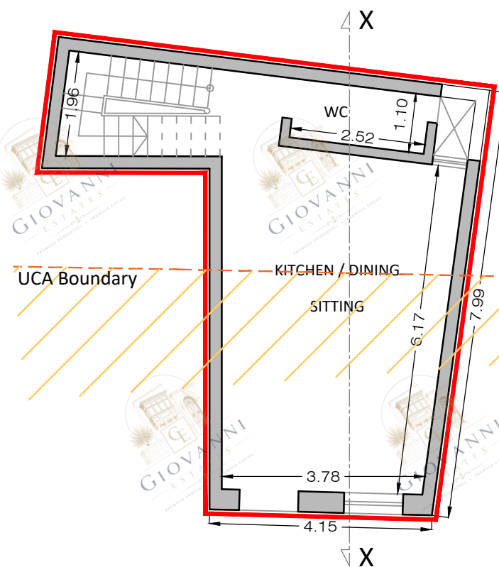
GROUND FLOOR PROPOSED Scale 1:100
