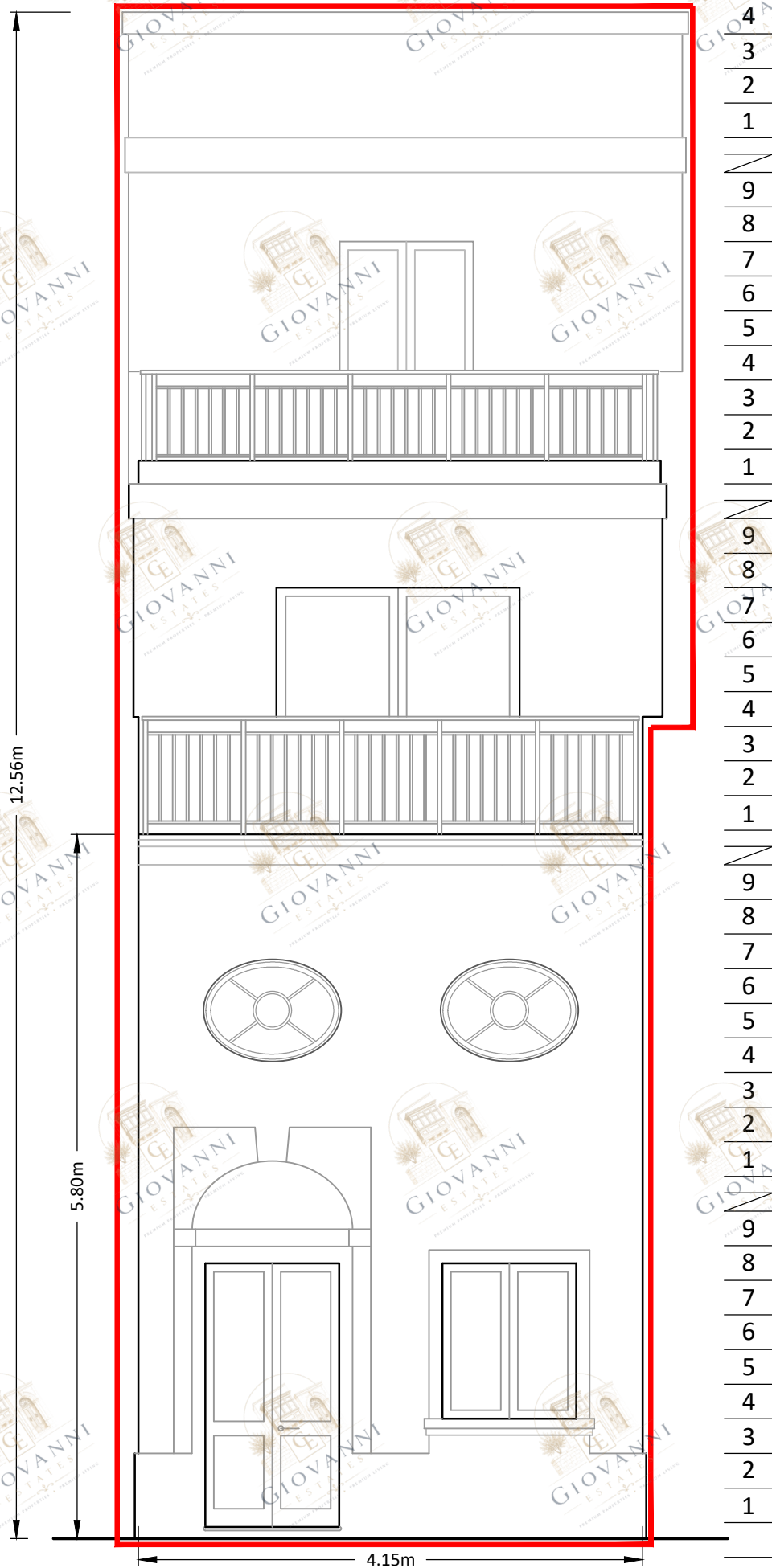
FRONT ELEVATION PROPOSED Scale 1:50
