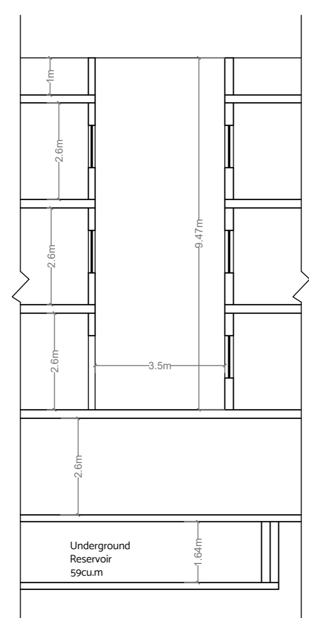
Proposed Sectional view Z-Z Scale 1:100 clean copy
