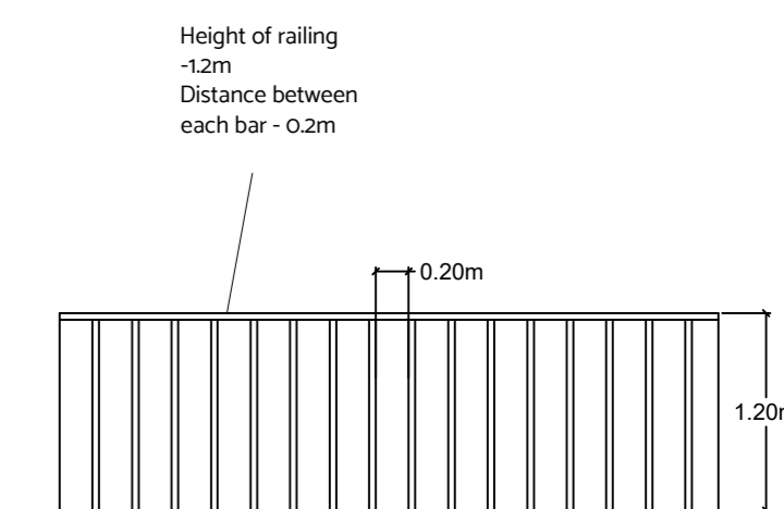
Proposed Elevation detail of gate through internal yard
