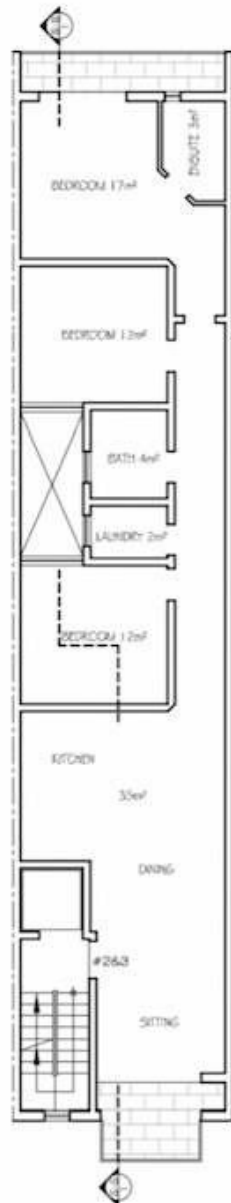
PROPOSED FIRST & SECOND FLOOR PLAN 1:100
