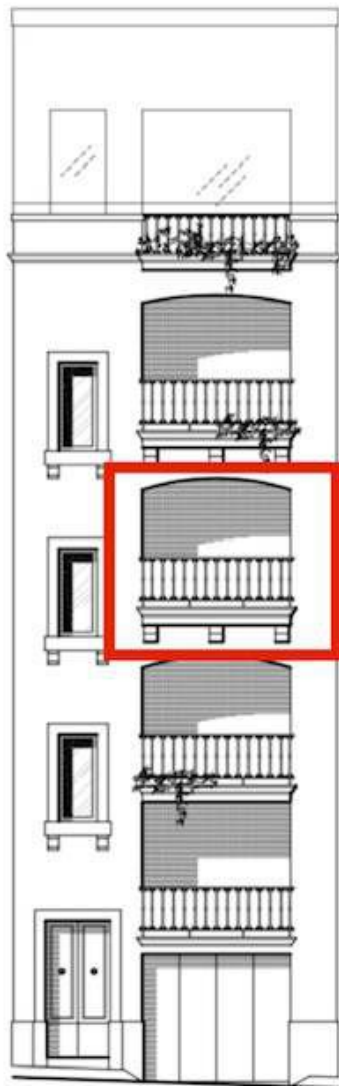
PROPOSED FRONT ELEVATION 1:100 unrendered franka stone facade white alum. apertures and railings
