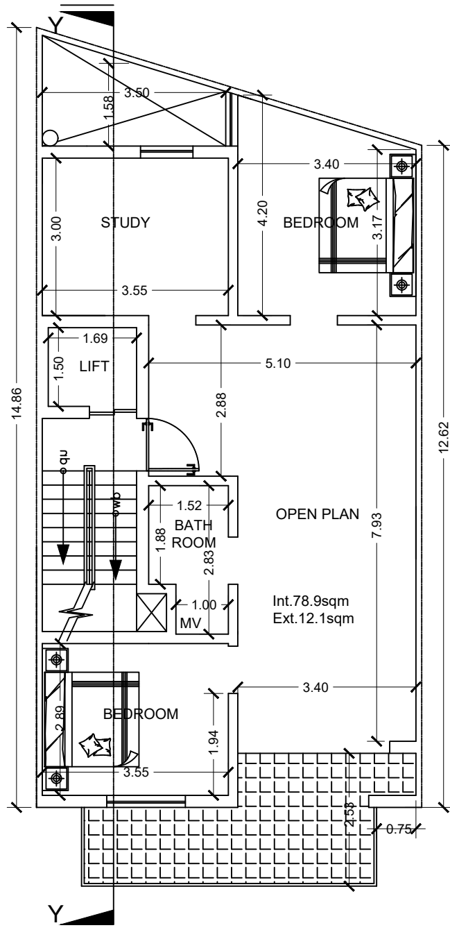
TYPICAL FLOOR - as proposed (clean copy) (levels 1 to 5) SCALE 1:100
