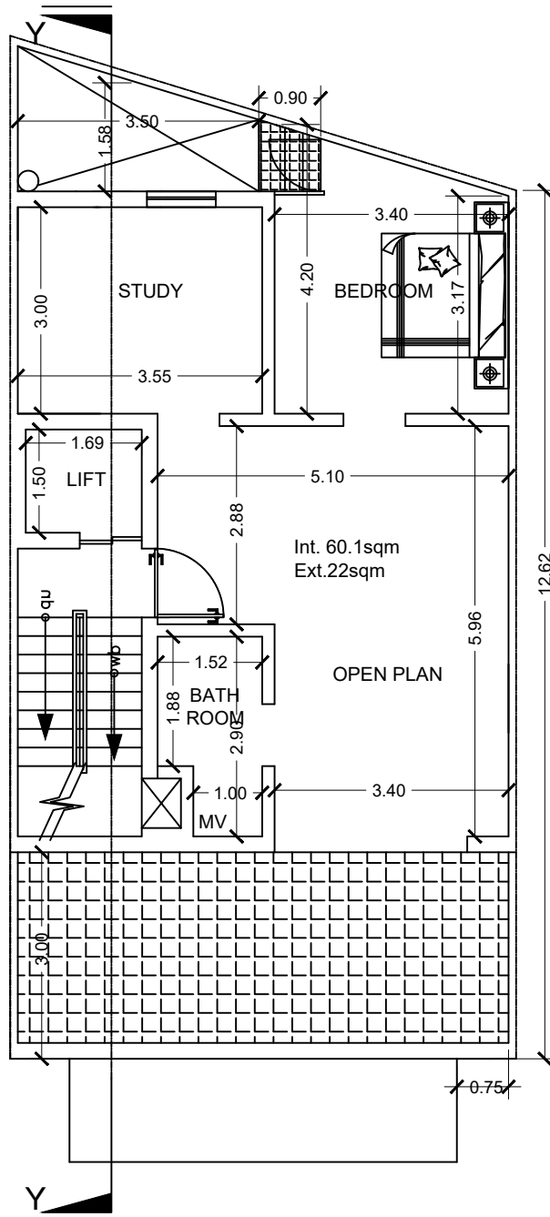
SIXTH FLOOR - as proposed (level 6) (clean copy) SCALE 1:100
