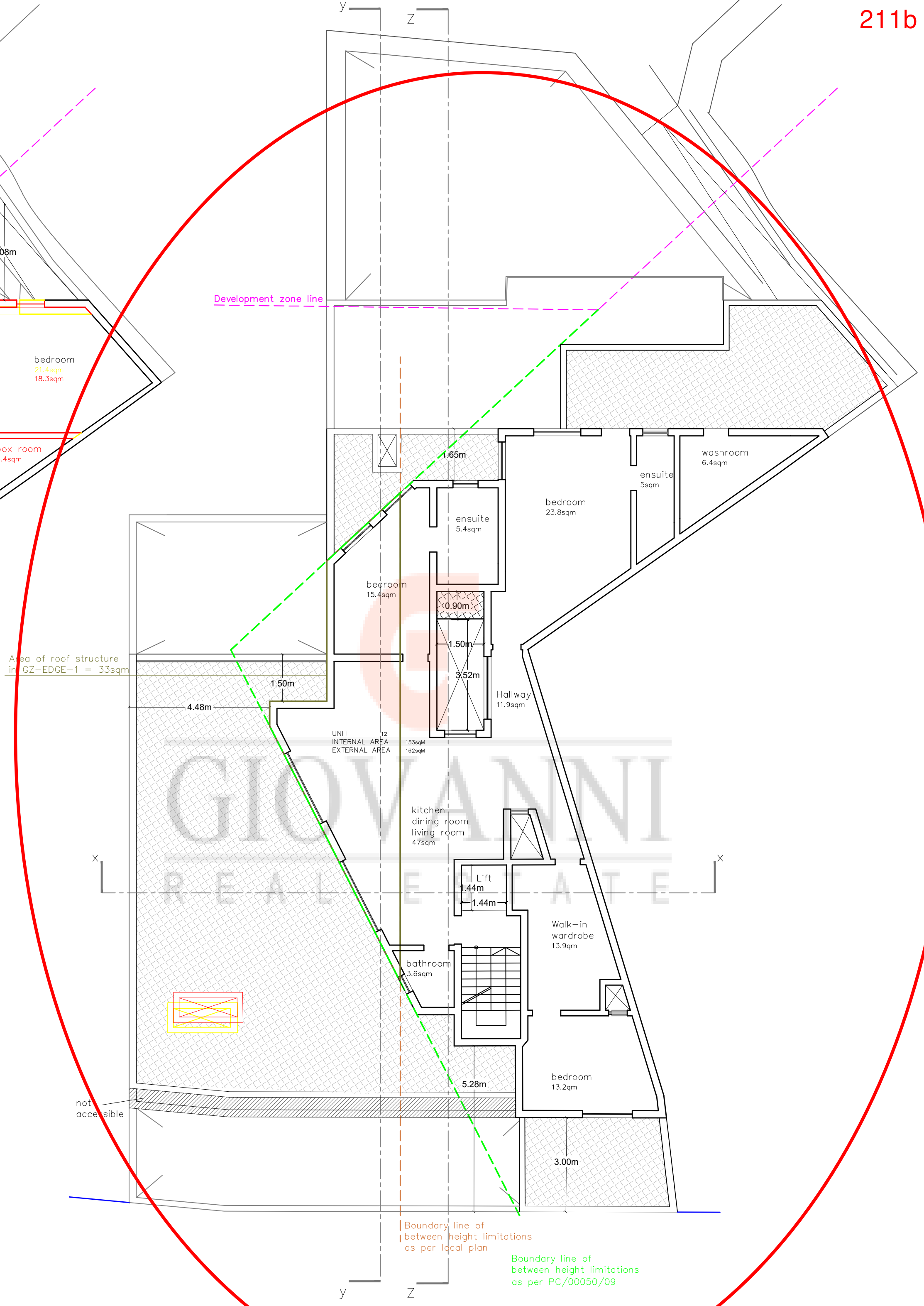
PROPOSED PENTHOUSE FLOOR LEVEL Scale 1:100
