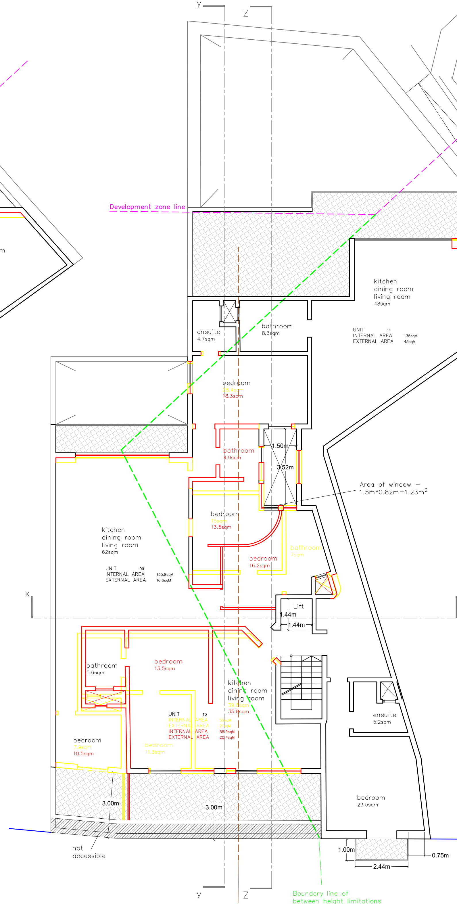
PROPOSED THIRD FLOOR LEVEL Scale 1:100
