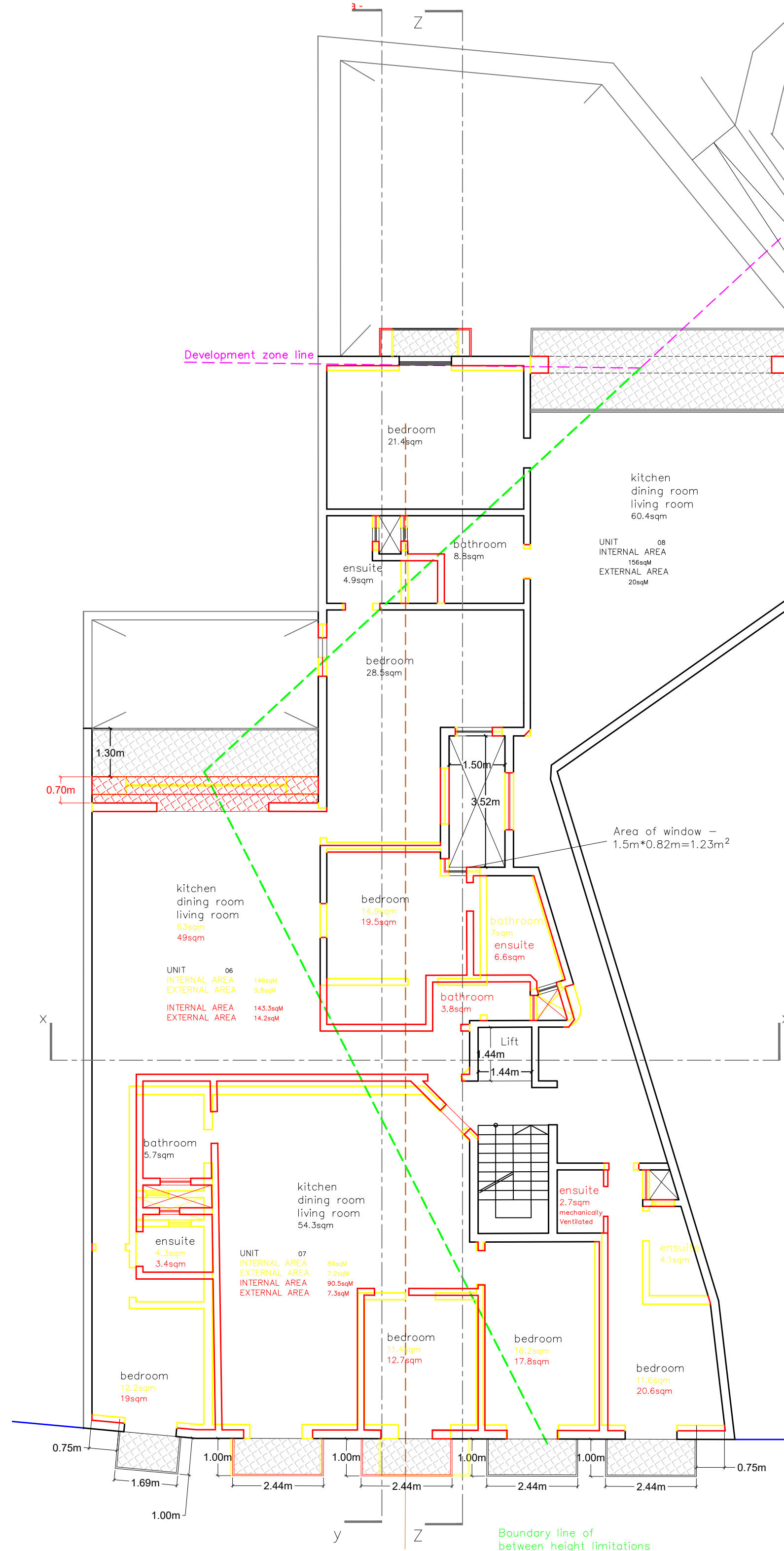
PROPOSED SECOND FLOOR LEVEL Scale 1:100
