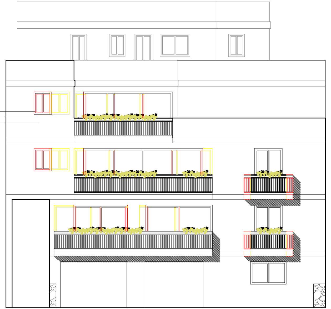
PROPOSED back elevation Scale 1:100
