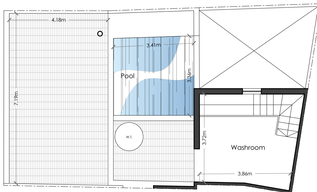
Roof Level Scale 1:100
