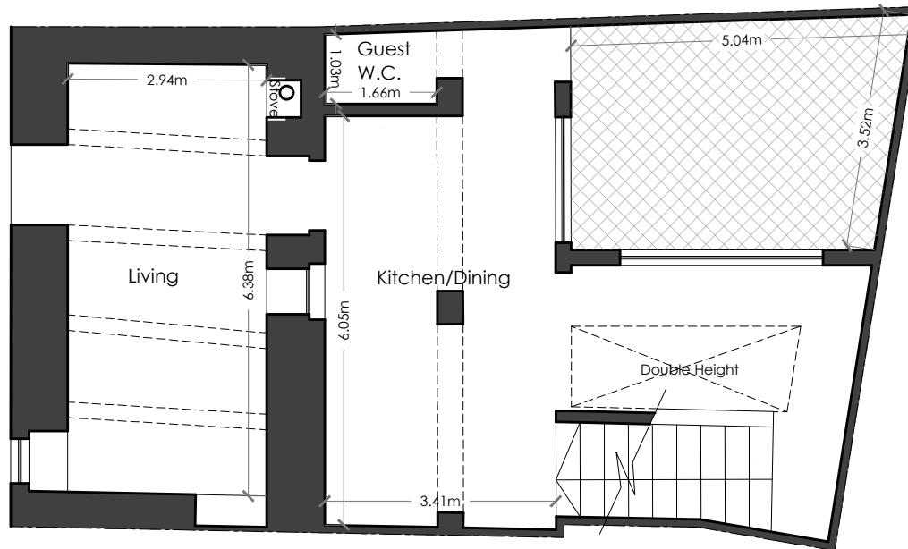
Ground Floor Level Scale 1:100
