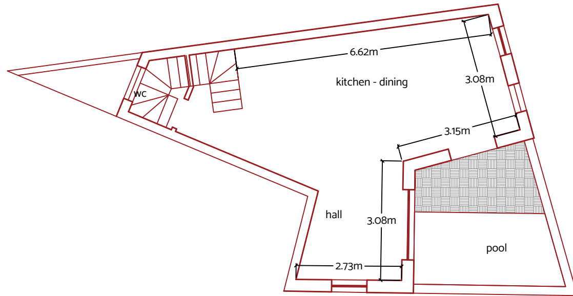
Proposed Ground Floor Scale 1:100 clean copy
