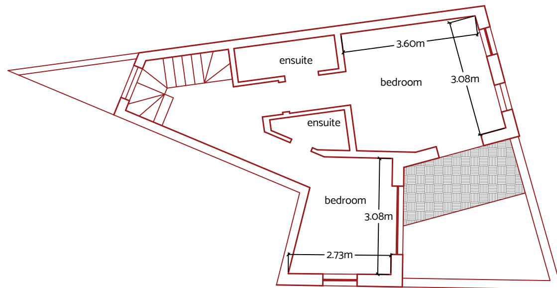
Proposed second Floor Scale 1:100 clean copy
