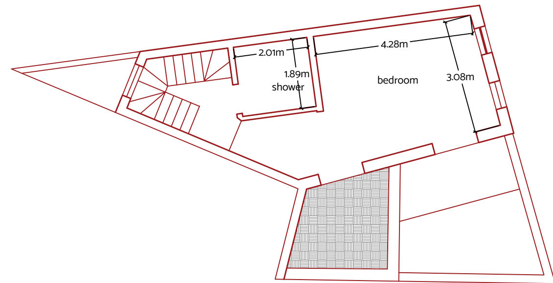
Proposed receded Floor Scale 1:100 clean copy
