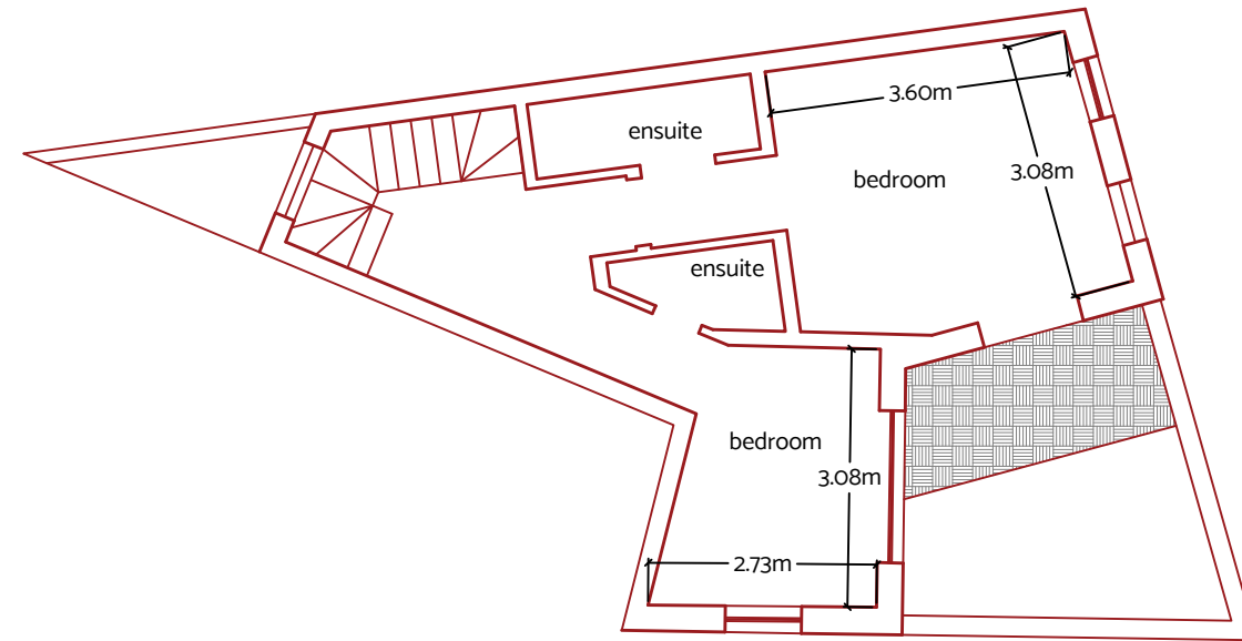
Proposed First Floor Scale 1:100 clean copy
