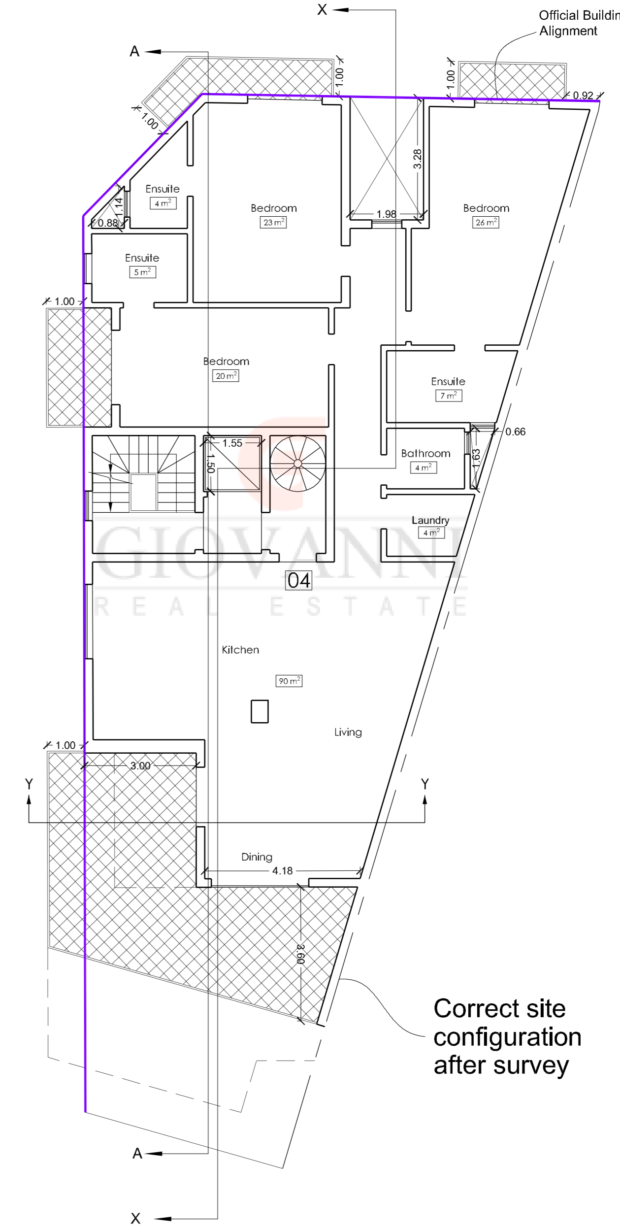
Proposed Second Floor
