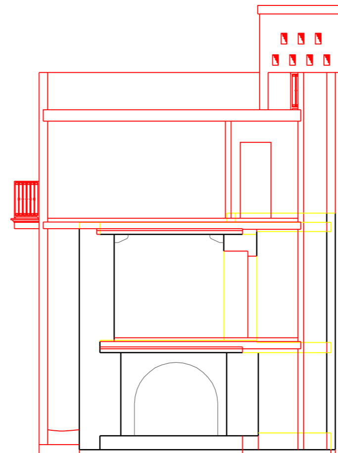
Existing & Proposed Section Y-Y
