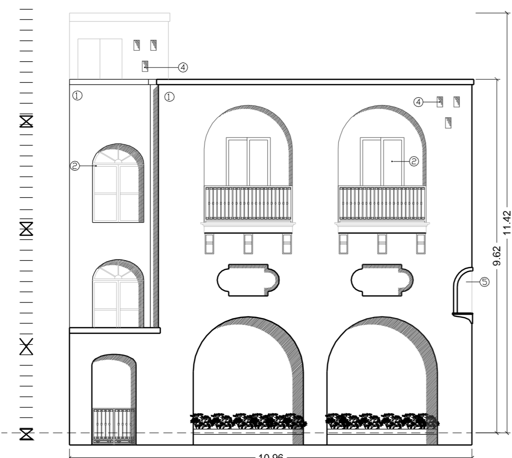
Proposed Facade A
