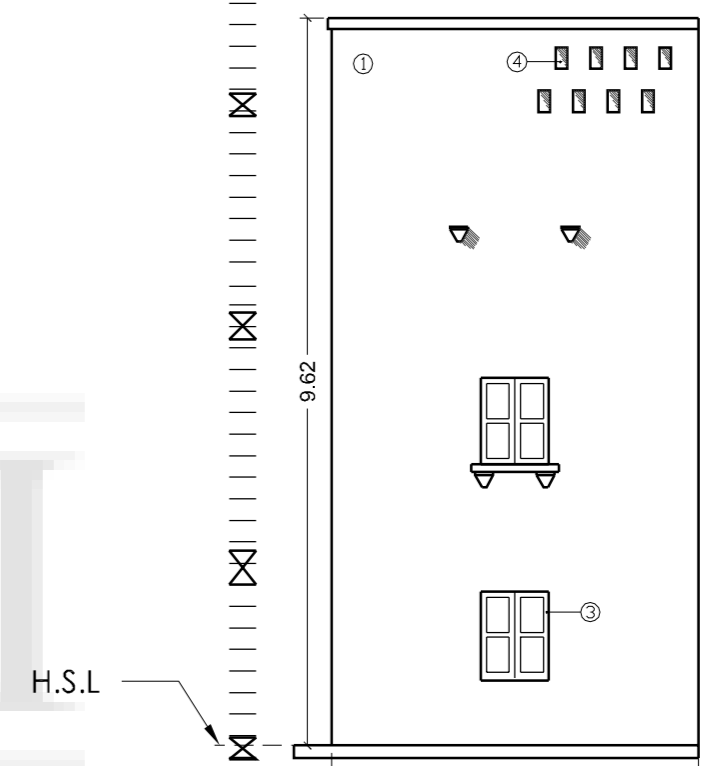
Proposed Facade C
