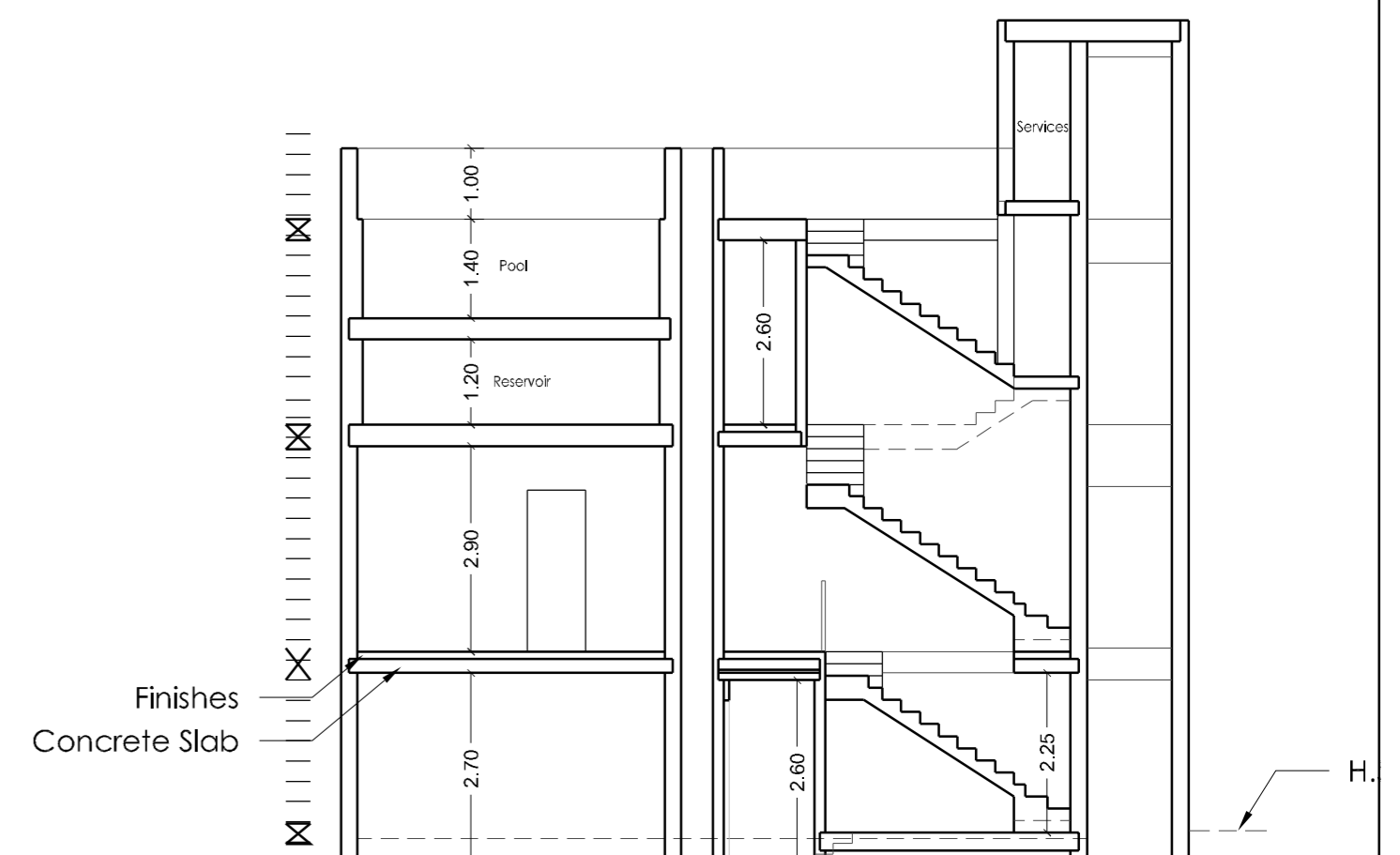
Proposed Section X-X
