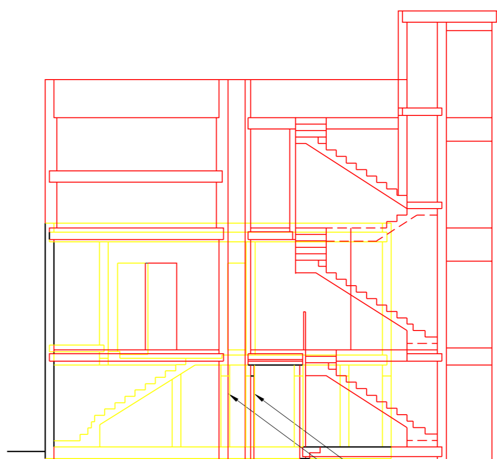
Existing & Proposed Section X-X
