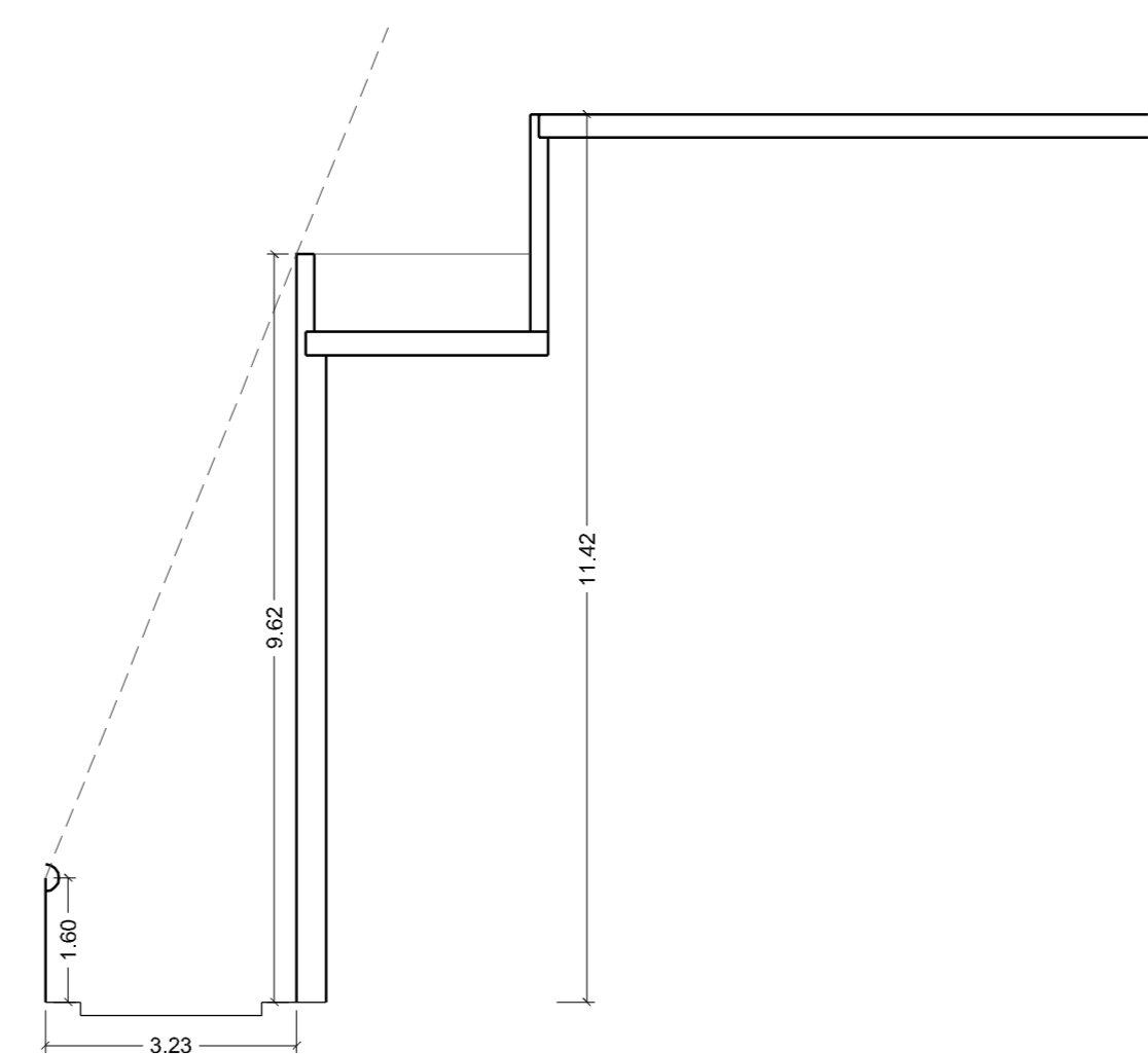
Proposed Section thru Street
