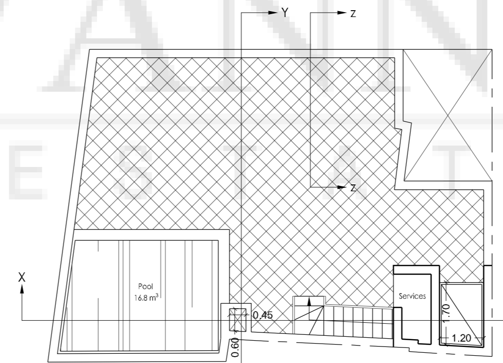
Proposed (clean copy) Roof Floor
