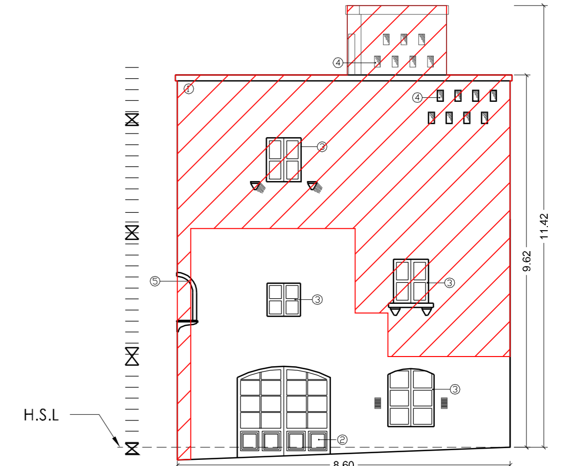
Proposed Facade B
