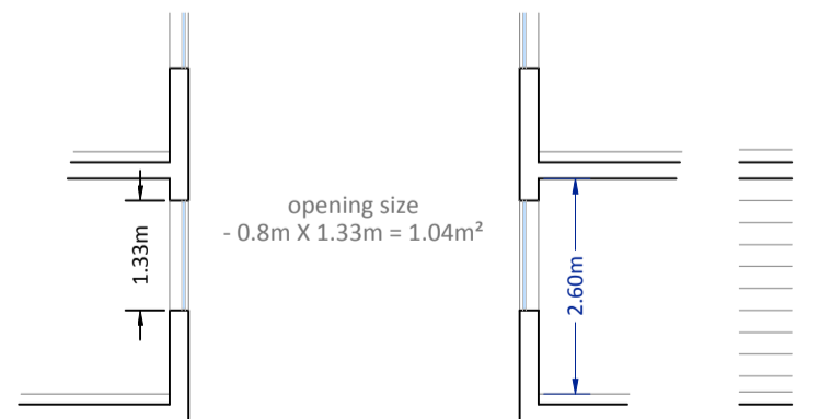
Proposed part section through a typical bedroom window overlooking the internal yard scale 1:100
