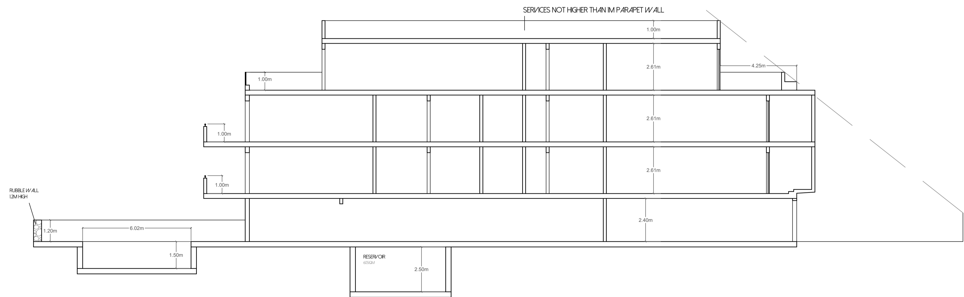
PROPOSED SECTION X-X SCALE 100 CLEAN COPY
