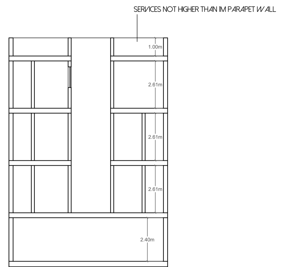
PROPOSED SECTION Y-Y SCALE 100 CLEAN COPY
