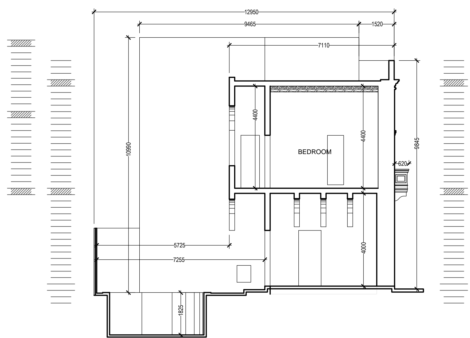
EXISTING SECTION BB Scale 1:100
