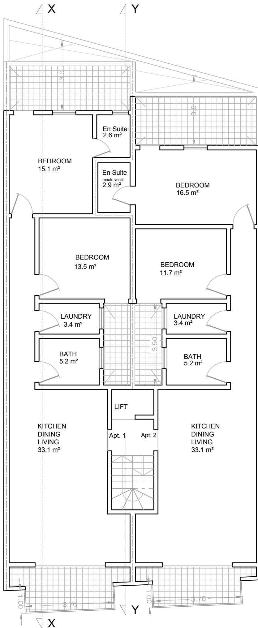
FIRST FLOOR LEVEL PLAN
