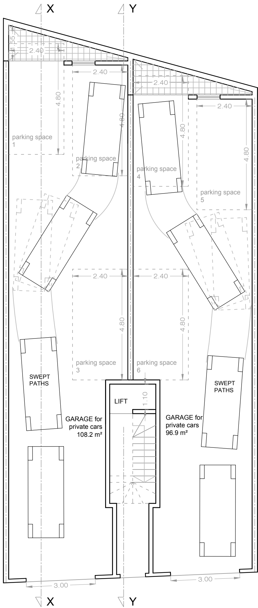
GROUND FLOOR LEVEL PLAN
