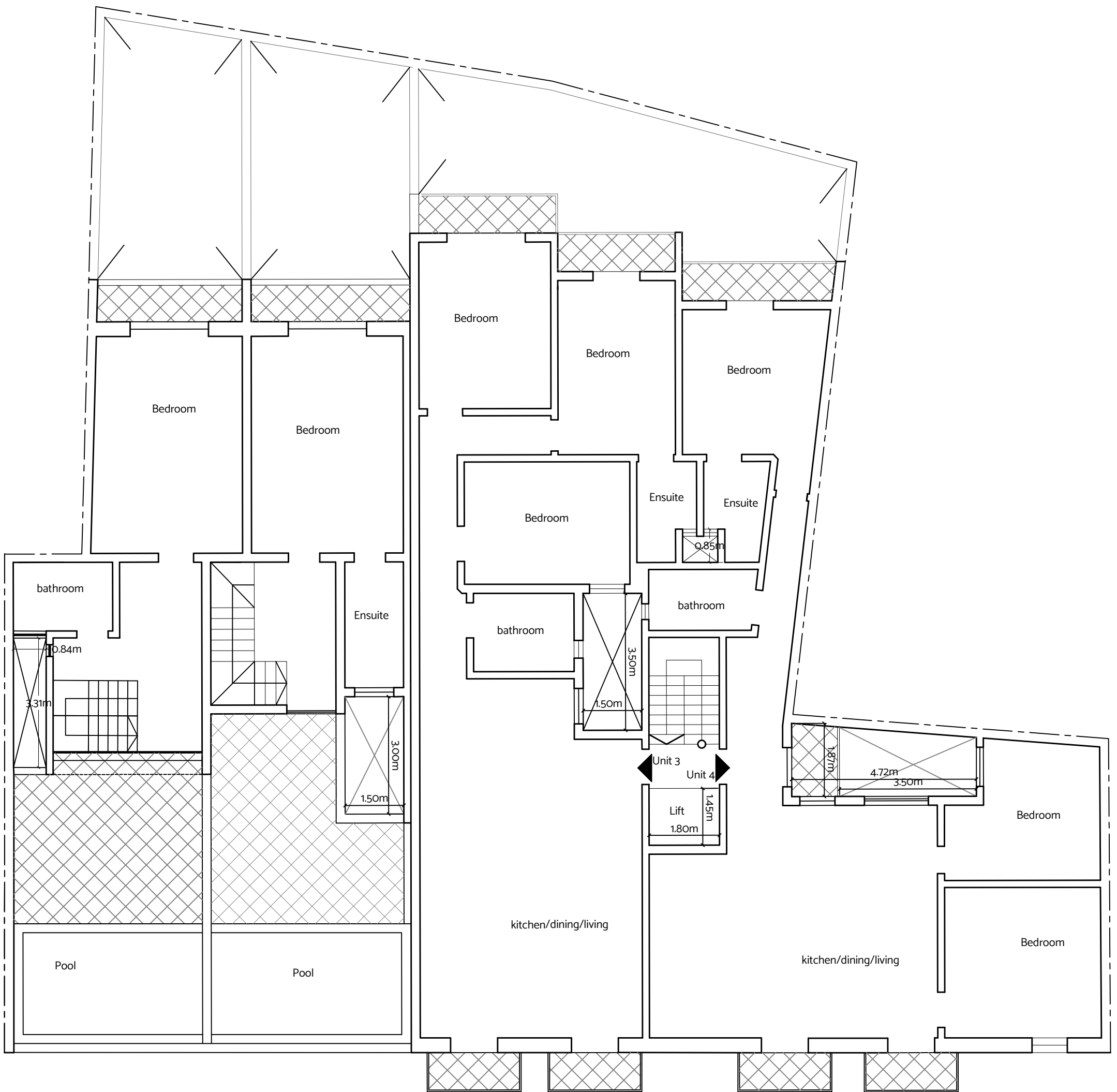
Proposed Second Floor Level Plan Scale 1:100 clean copy
