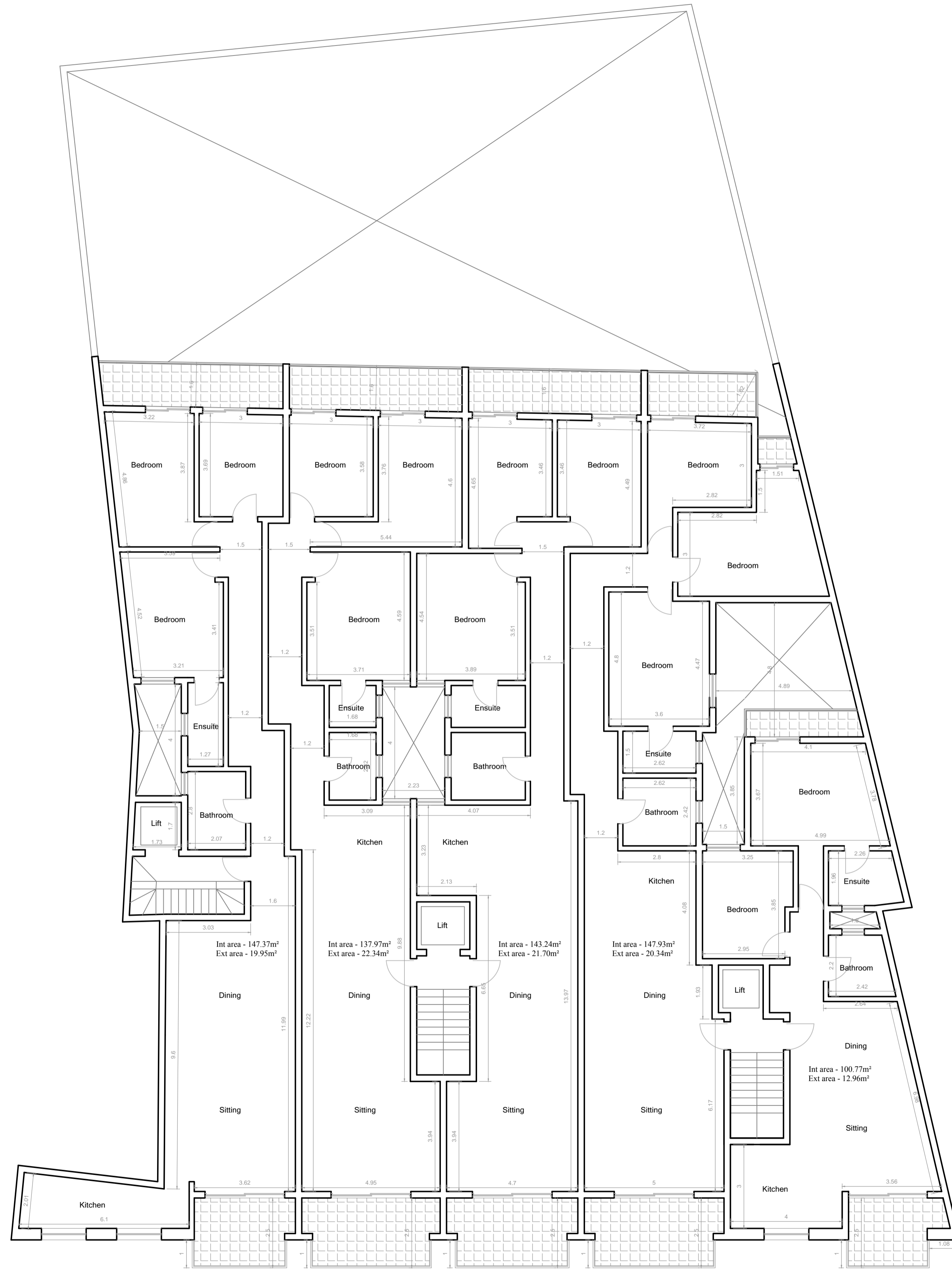
P5 D3 Proposed Third floor Scale 1:100
