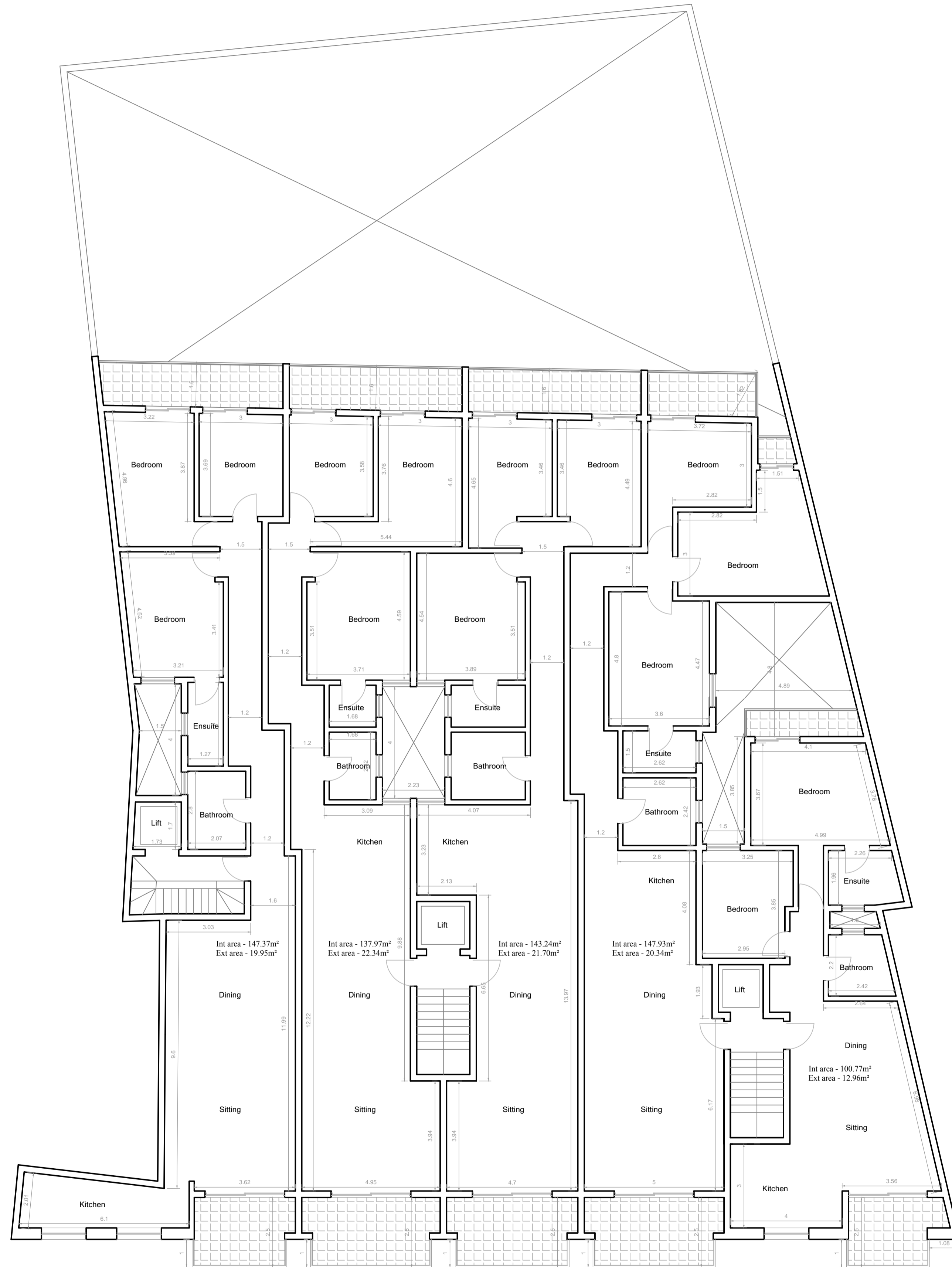
P3 D2 Proposed First floor Scale 1:100
