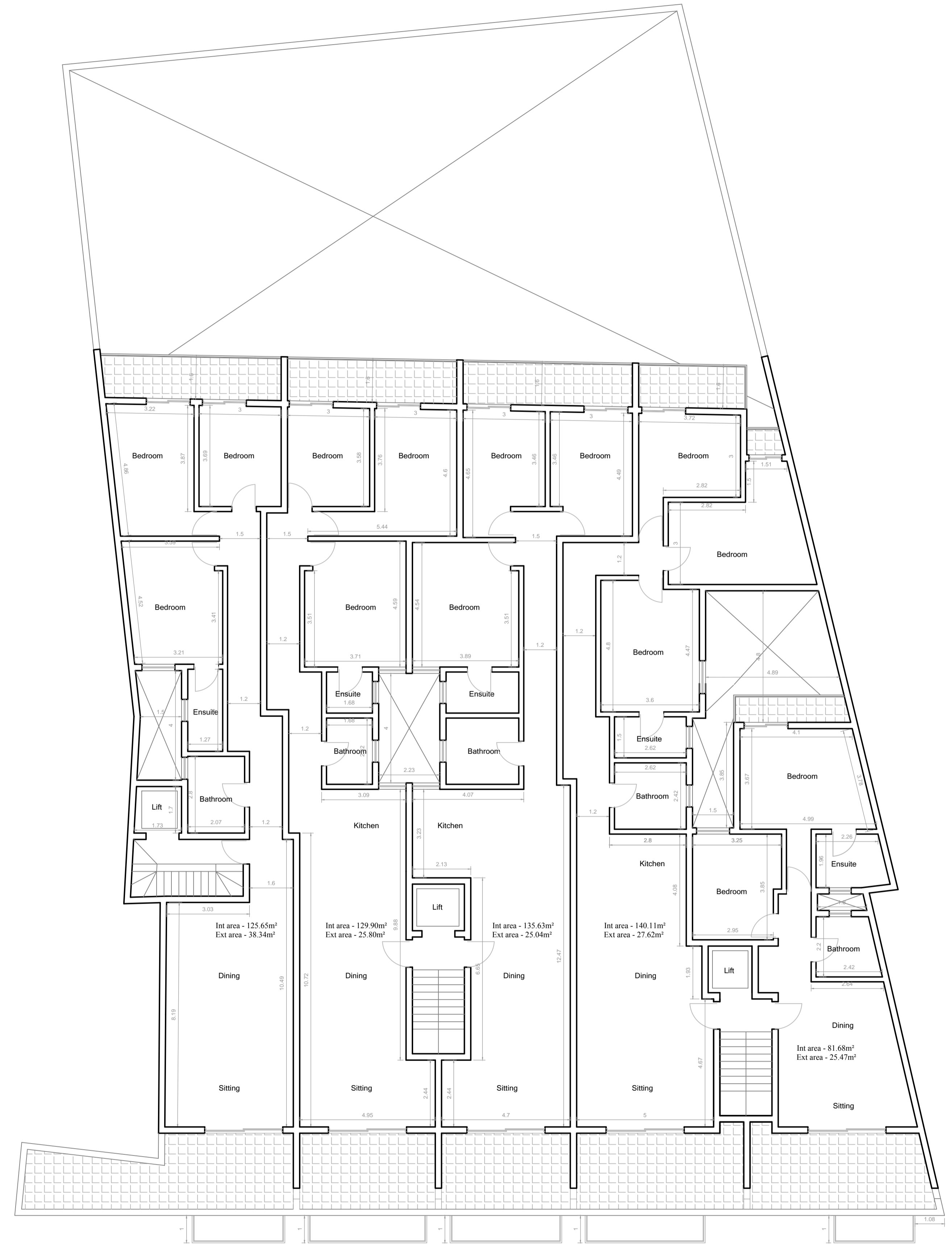
P6 D3 Proposed Penthouse floor Scale 1:100
