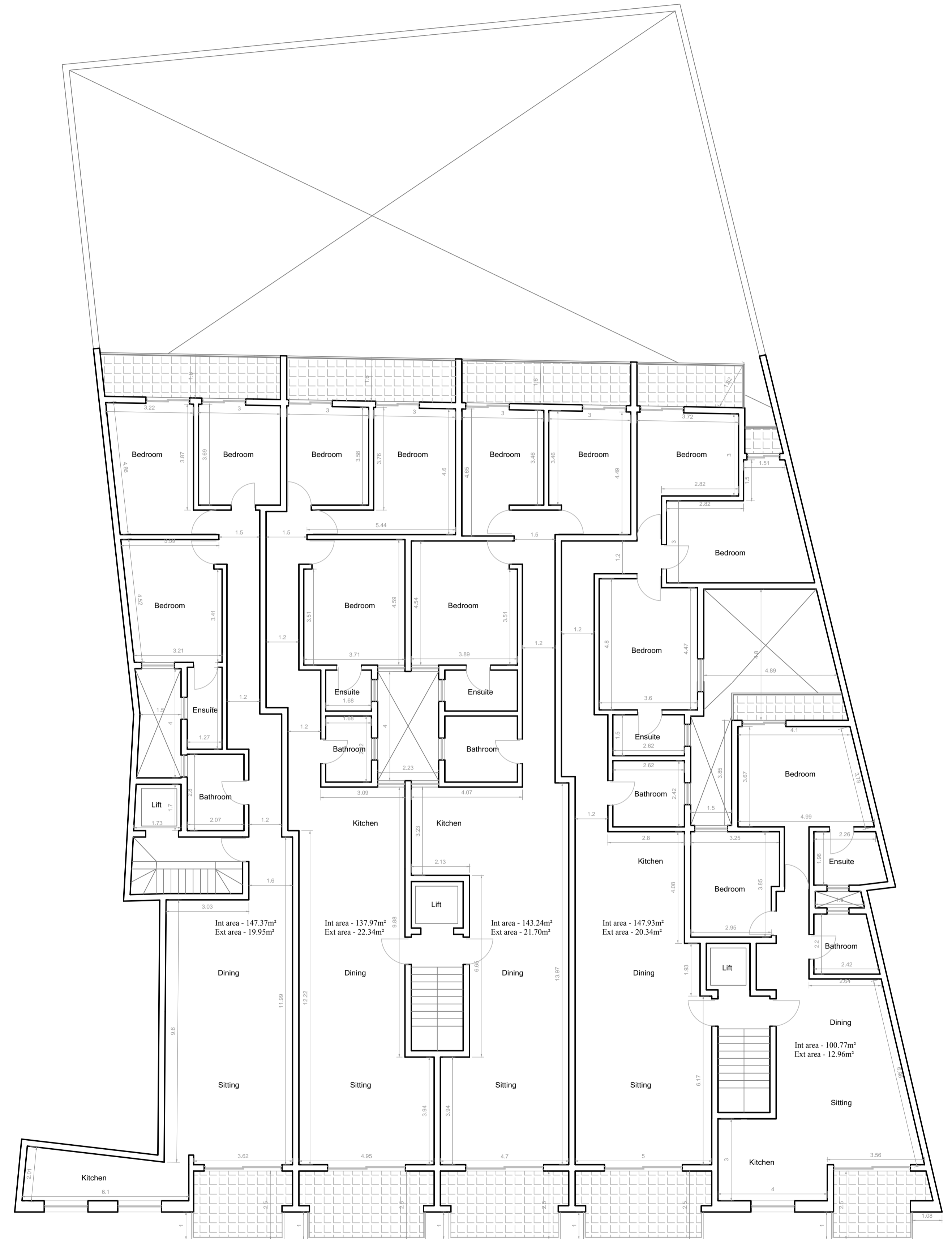
P4 D2 Proposed Second floor Scale 1:100
