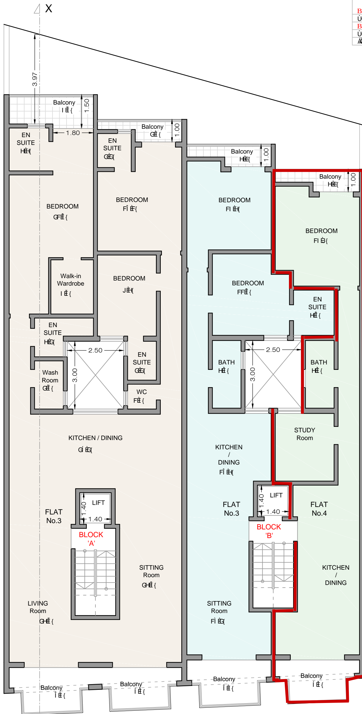
SECOND FLOOR Scale 1:100
