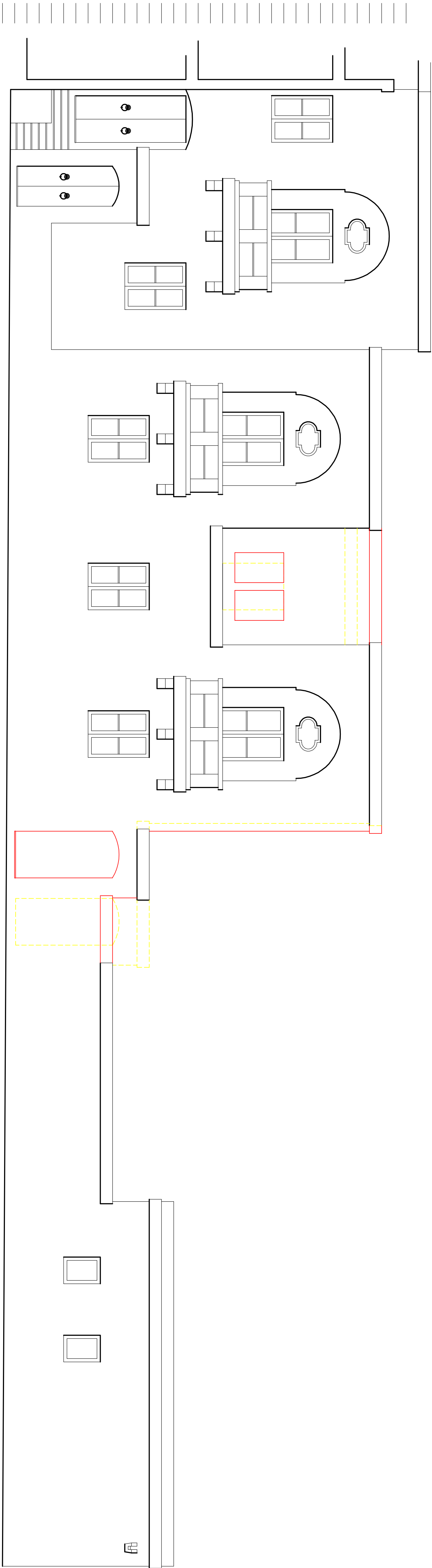
ELEVATION Q 1:50 / As Approved stone facade timber apertures painted blue
