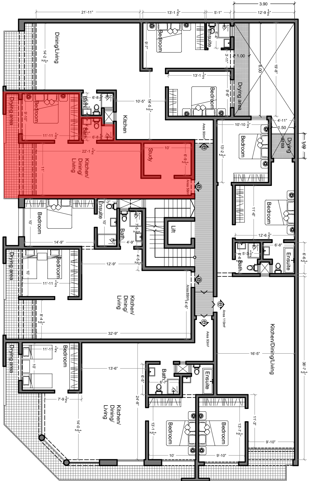
Proposed Typical Floor plan (2nd, 3rd, 4th floors) Scale: 1:100
