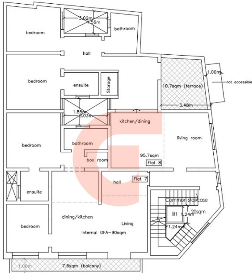
THIRD FLOOR AS PROPOSED scale 1:100
