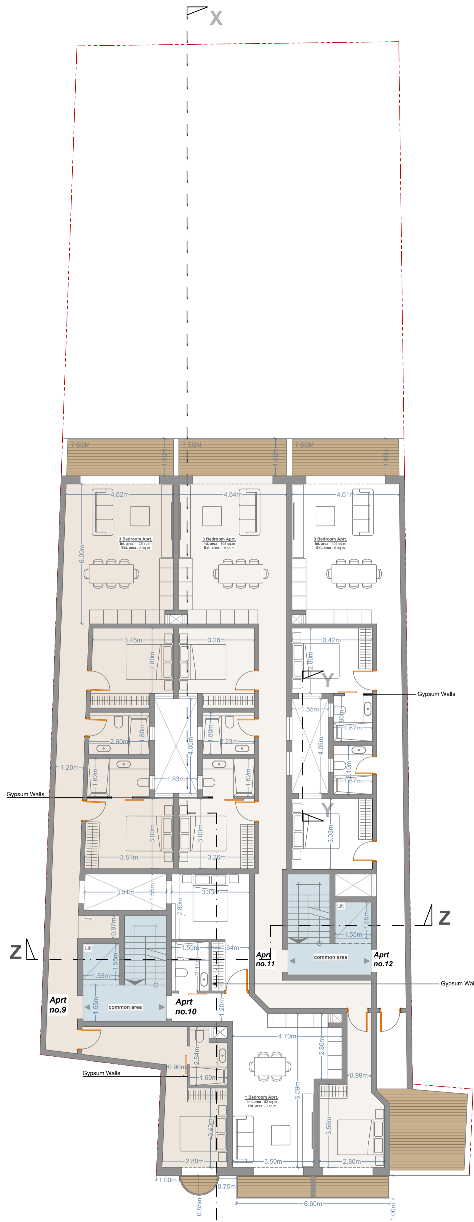
PROPOSED LEVELS 03 4 apartments scale 1:100
