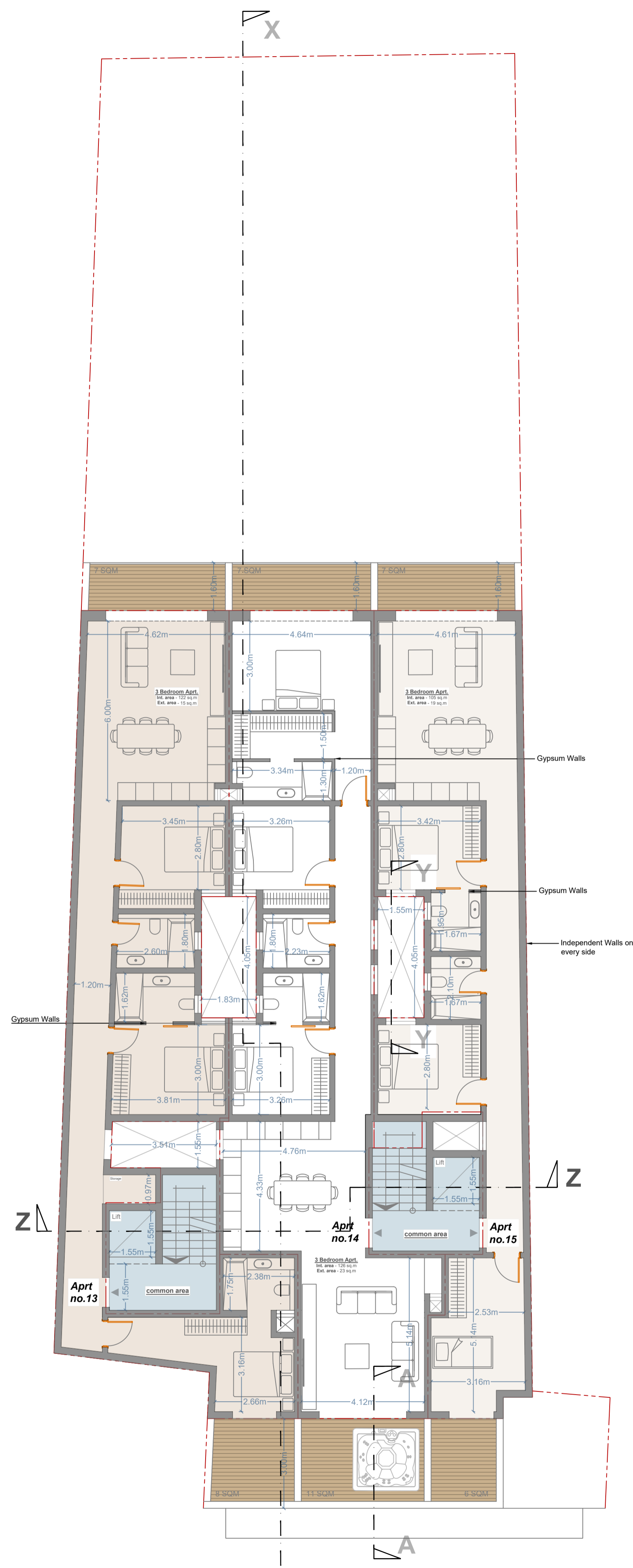
PROPOSED LEVEL 04 3 penthouses scale 1:100
