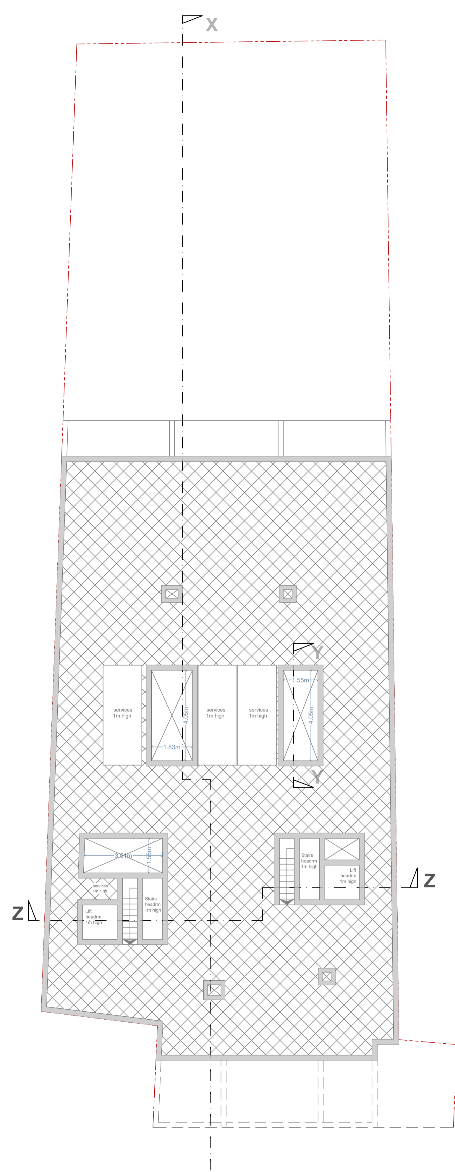
PROPOSED ROOF LEVEL scale 1:100
