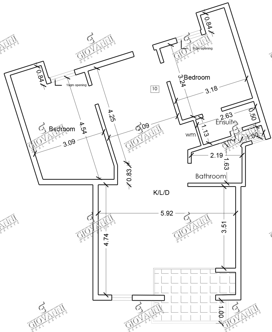
Proposed Third Floor (clean copy)
