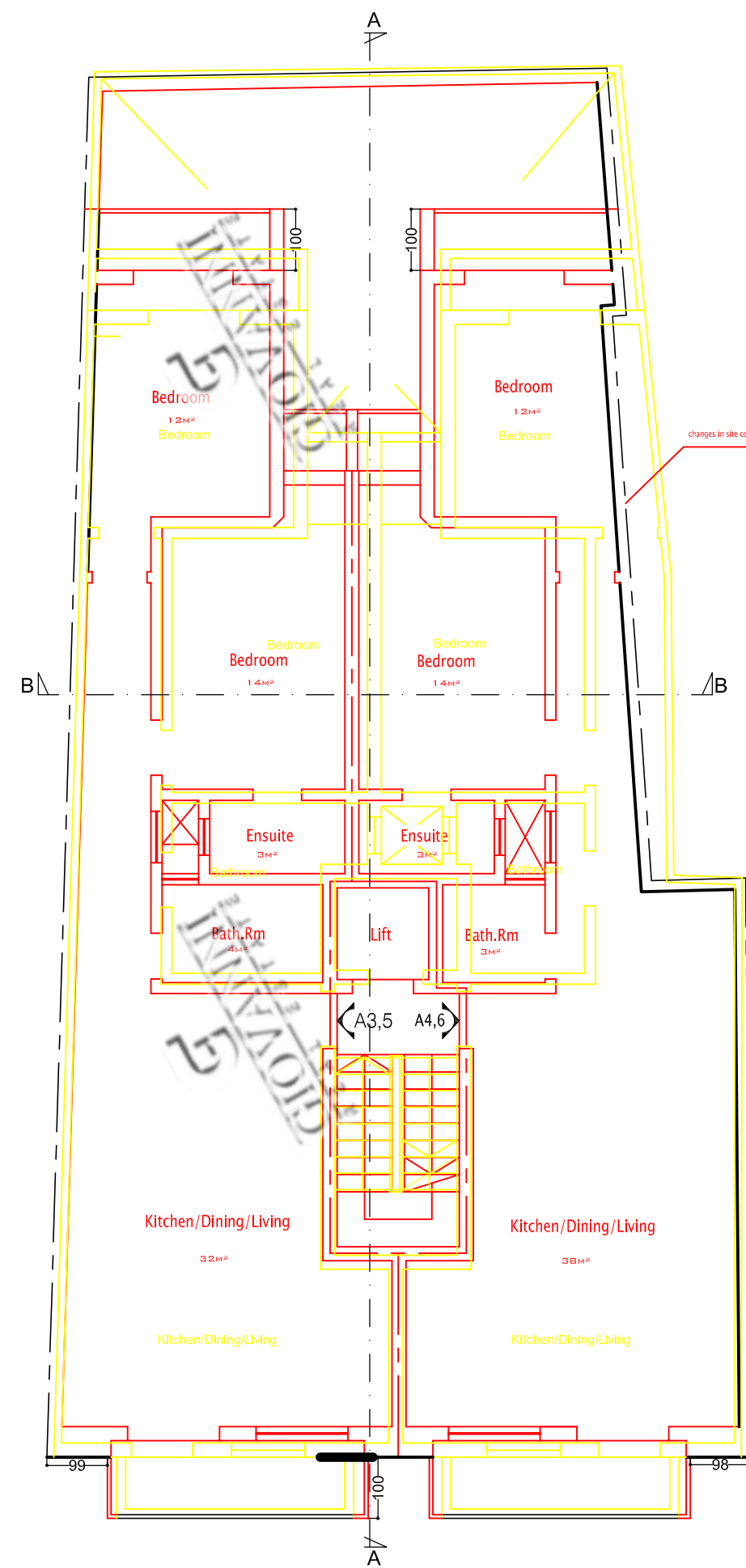
2nd and 3rd Floor Plan 1:100 Not Approved / Not Proposed
