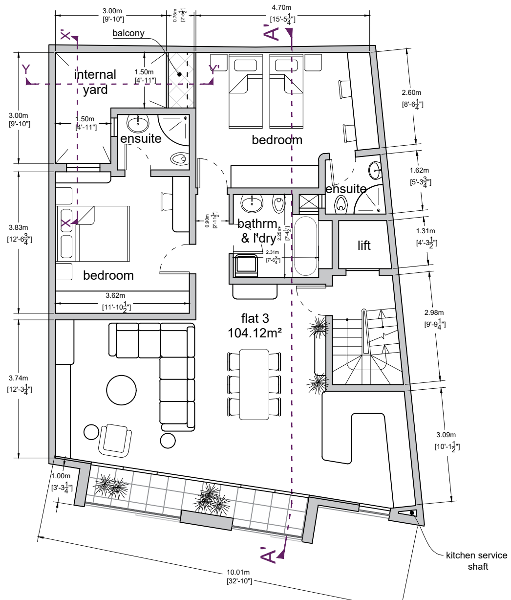
Thrid Floor Plan
