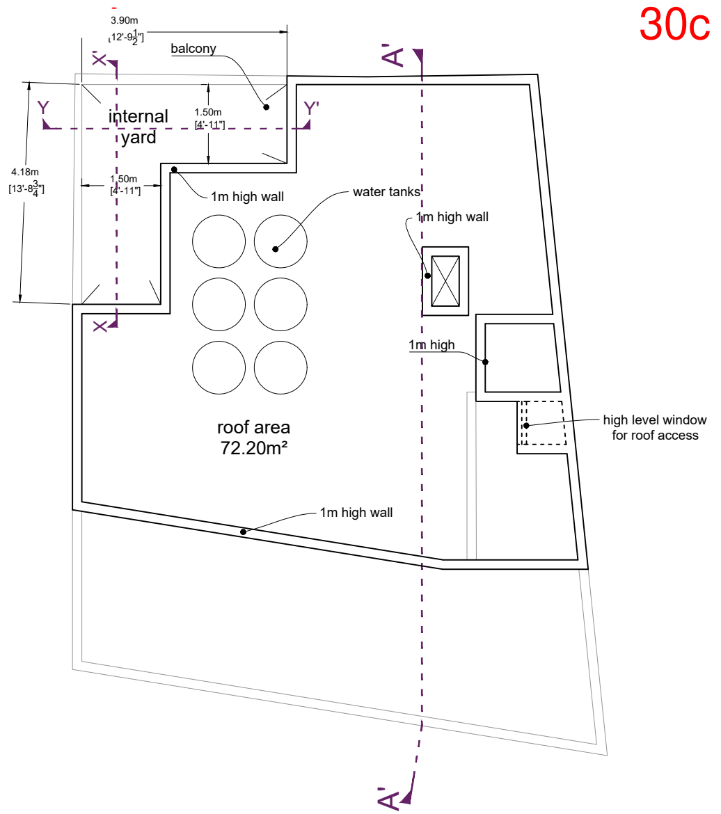
Roof Plan
