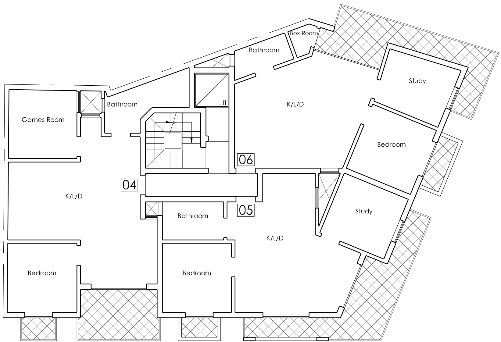
As Proposed Second Floor
