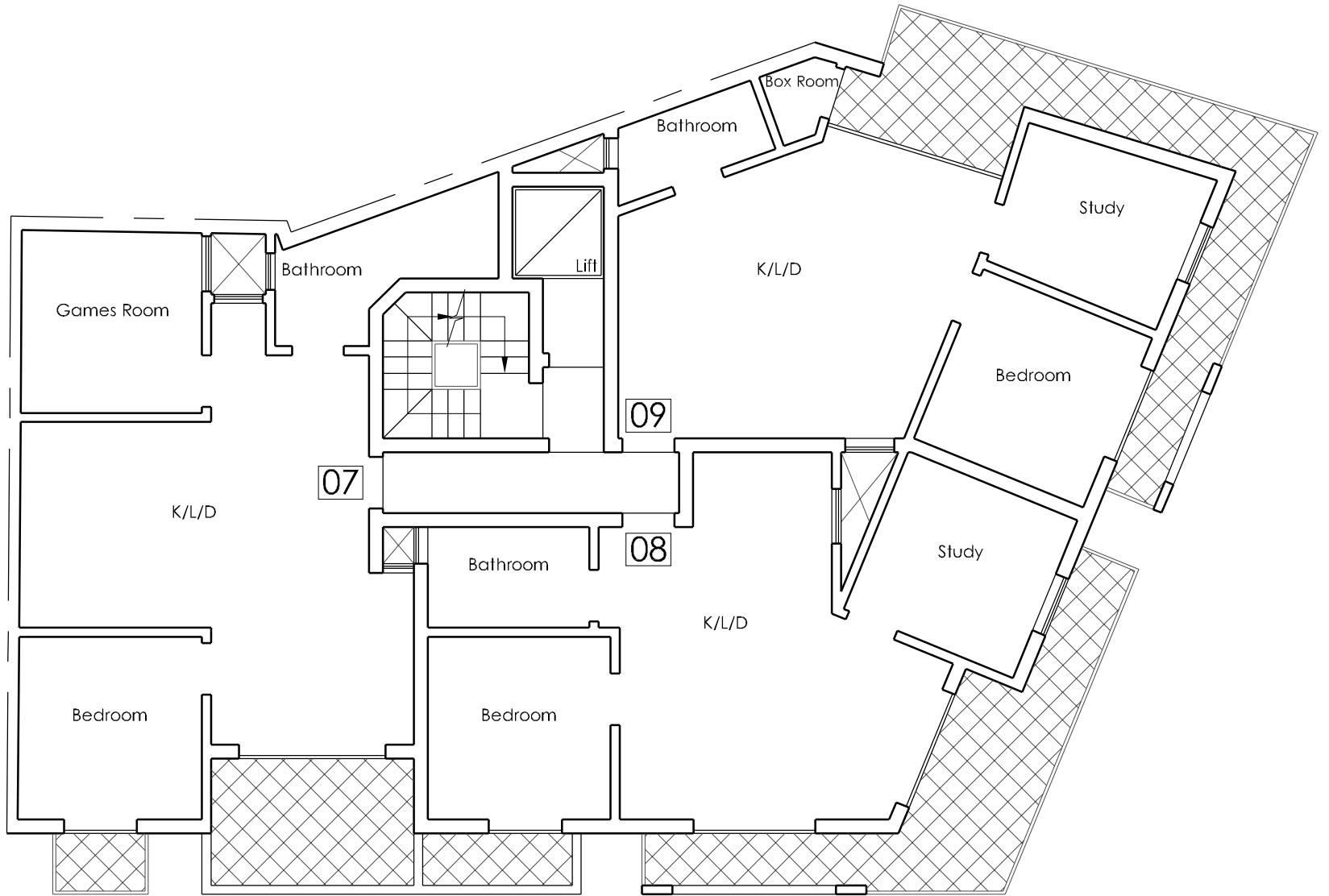
As Proposed Third Floor
