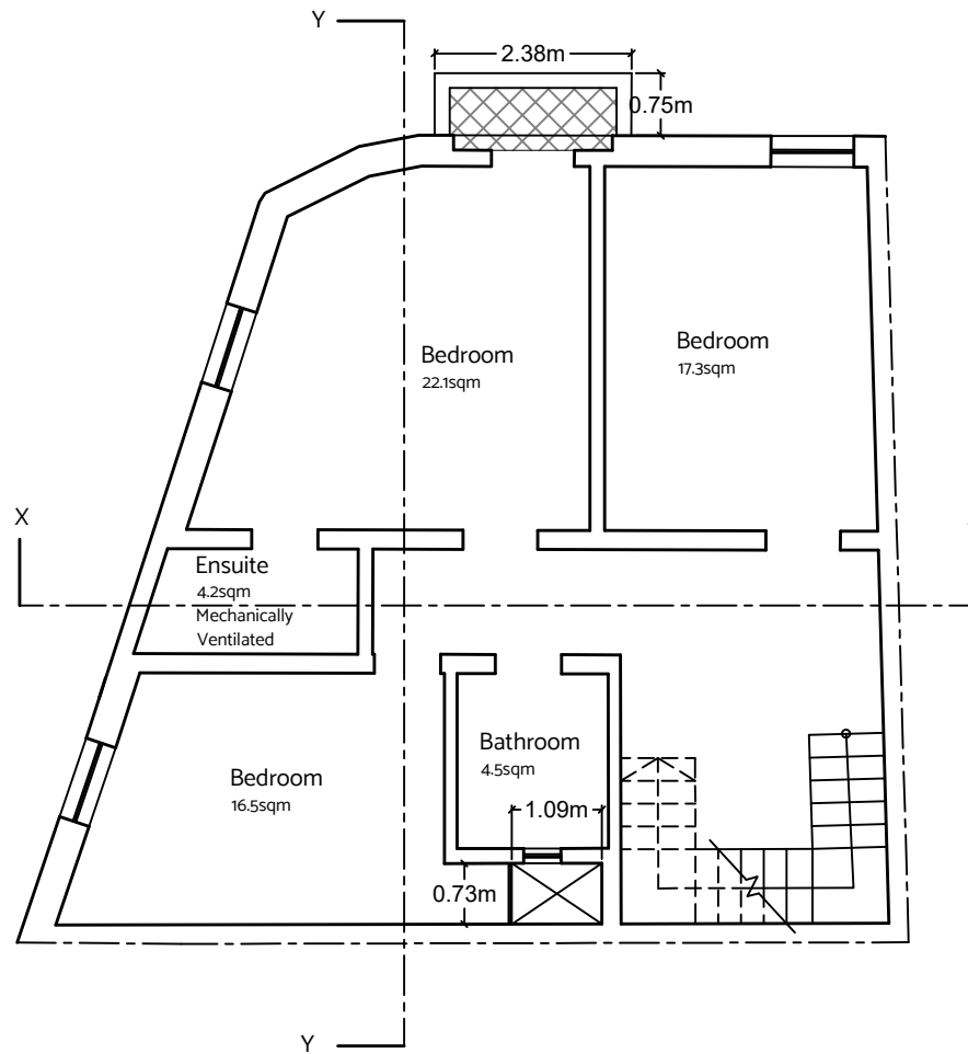
Proposed First Floor Level Plan Scale 1:100 clean copy
