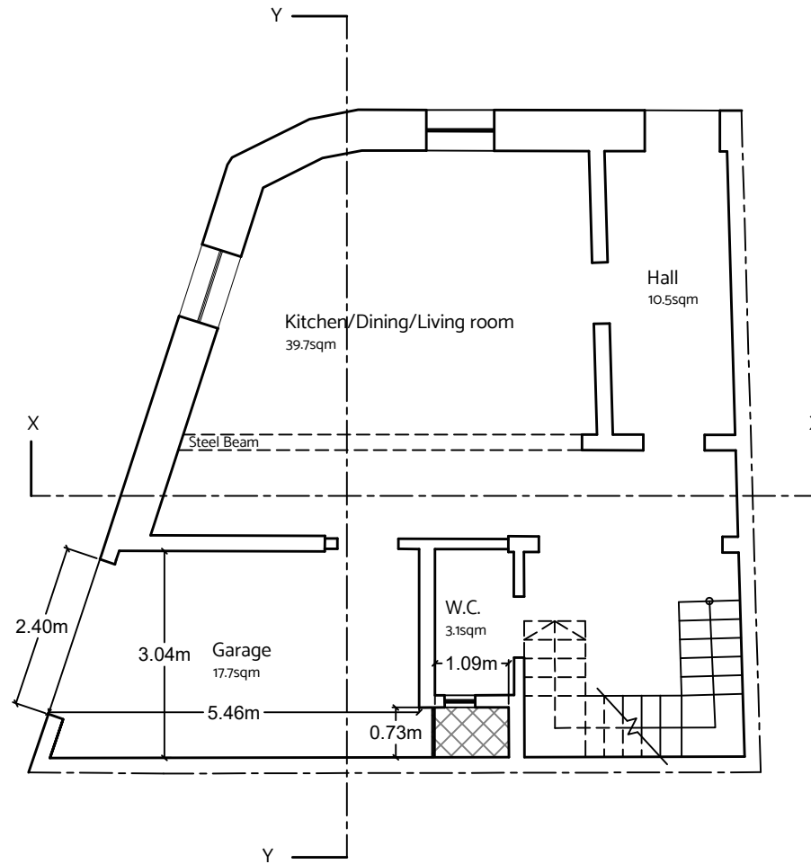
Proposed Ground Floor Level Plan Scale 1:100 clean copy
