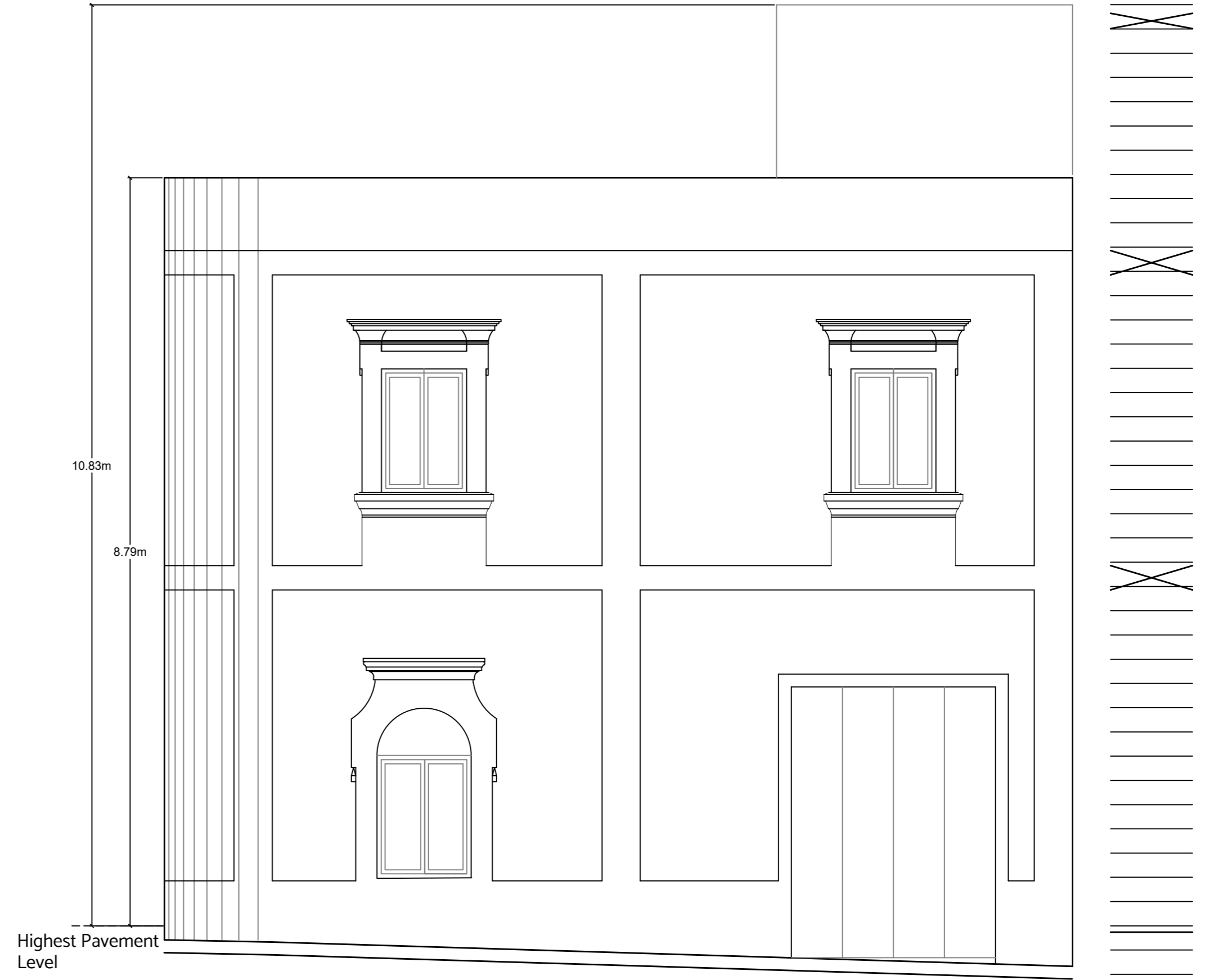
Proposed Elevation clean copy
