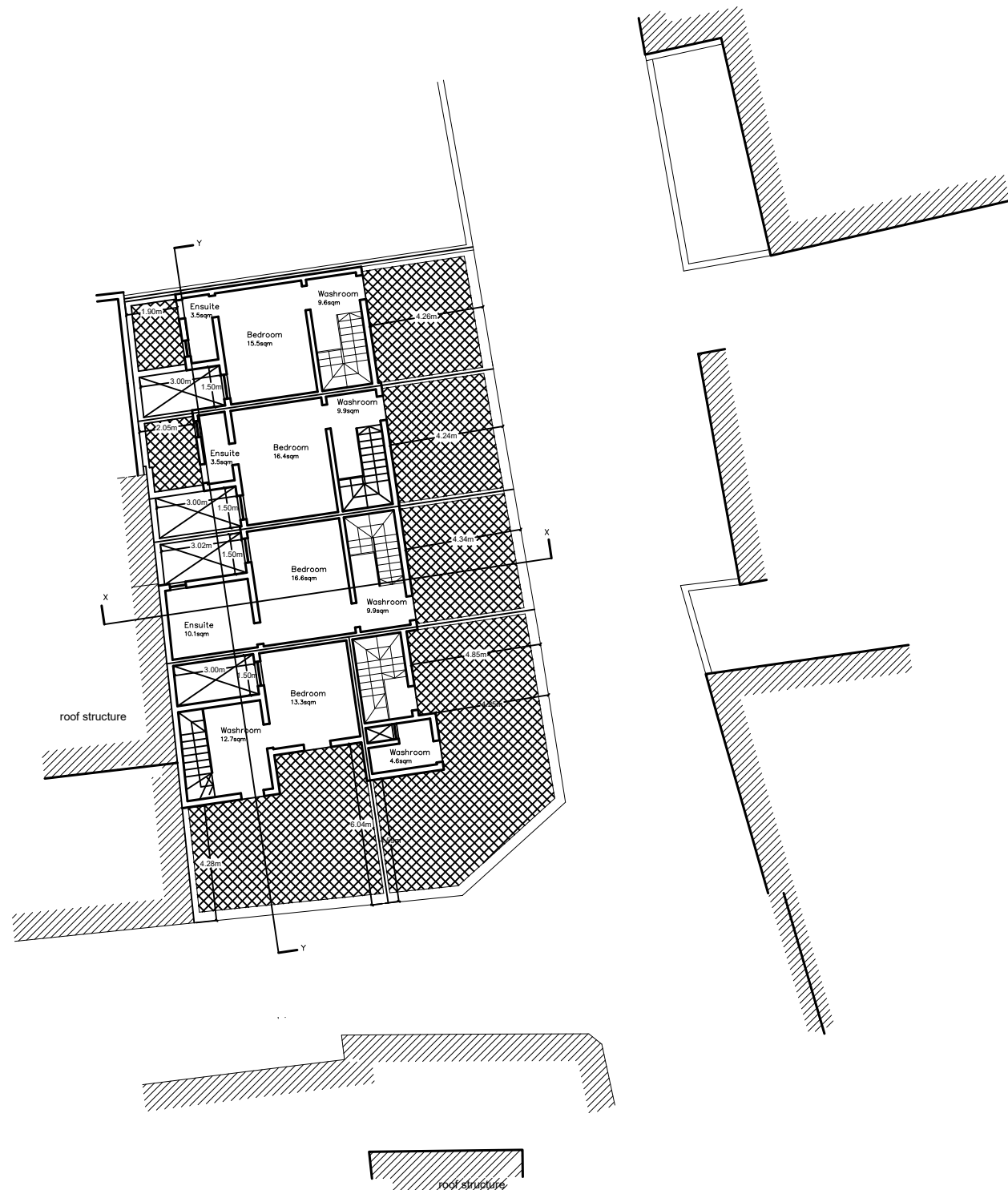
Proposed Roof Plan clean copy
