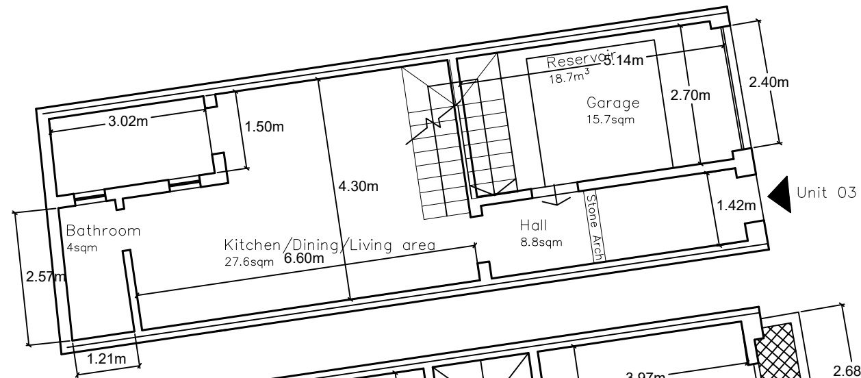
Proposed Ground Floor Level Plan Scale 1:100 clean copy
