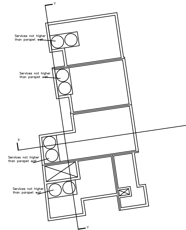
Proposed Upper Roof Plan clean copy
