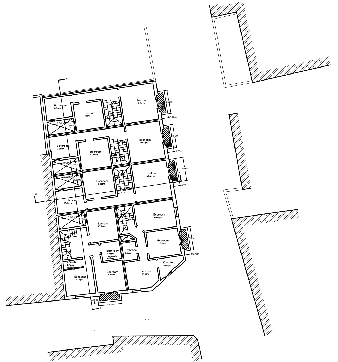
Proposed First Floor Level Plan Scale 1:100 clean copy
