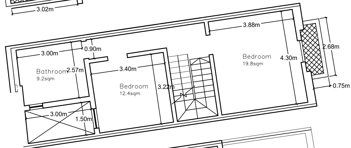
Proposed First Floor Level Plan clean copy Scale 1:100
