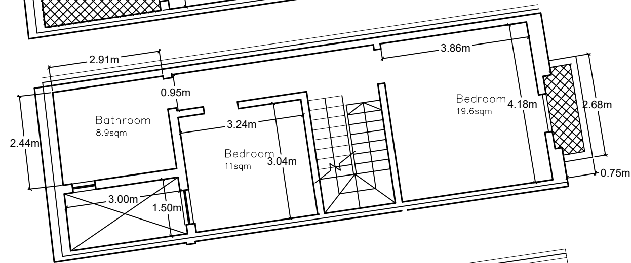
Proposed First Floor Level Plan Scale 1:100 clean copy
