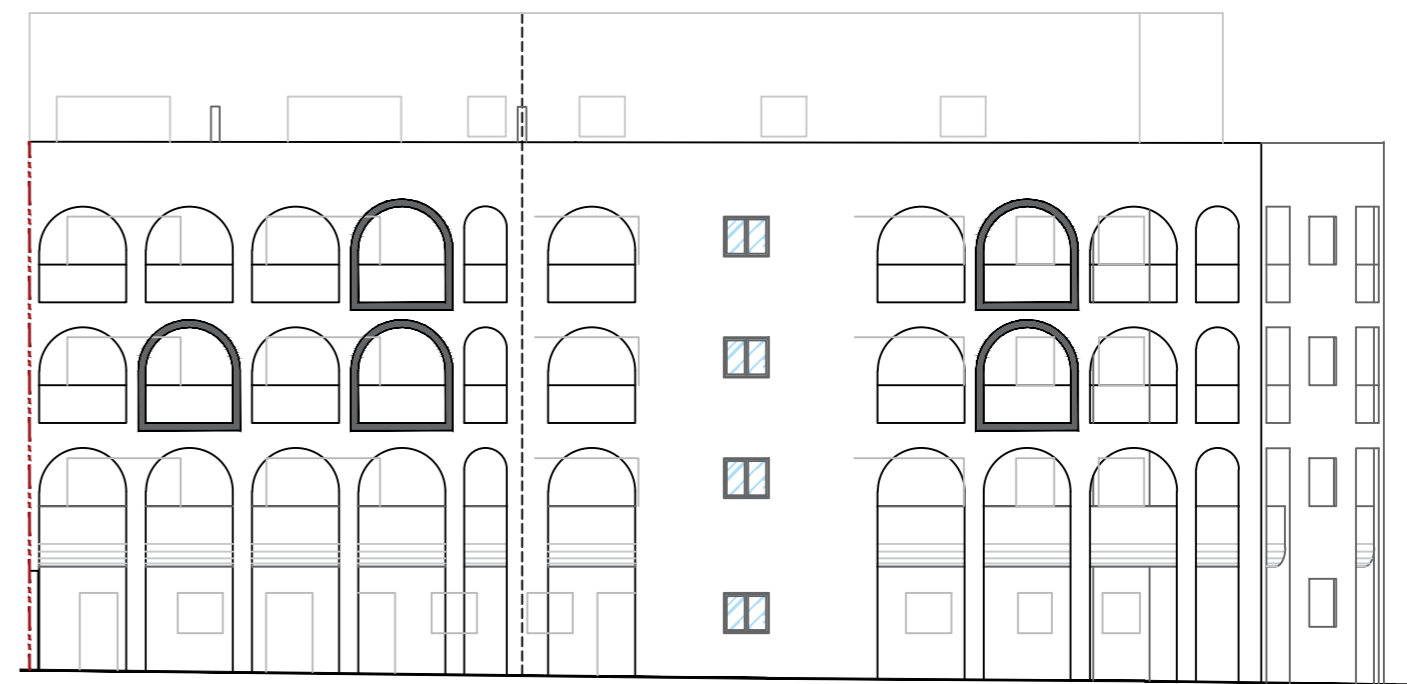
Proposed Internal Elevation D
