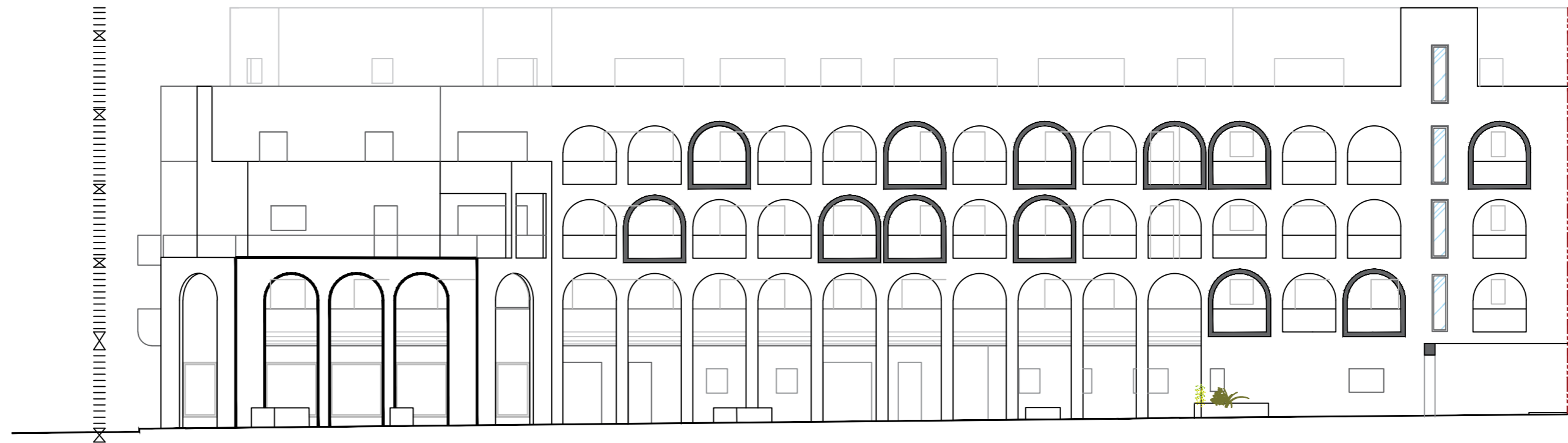
Proposed Internal Elevation A
