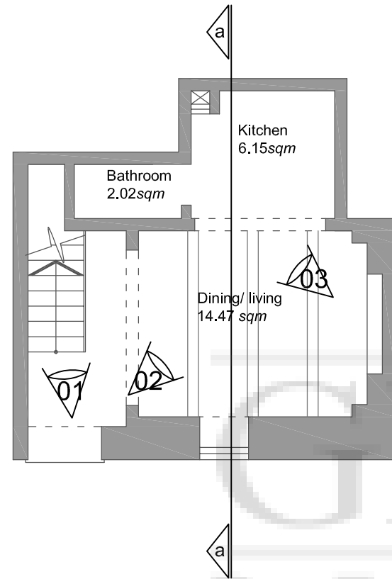
Ground Floor level existing Scale 1:100
