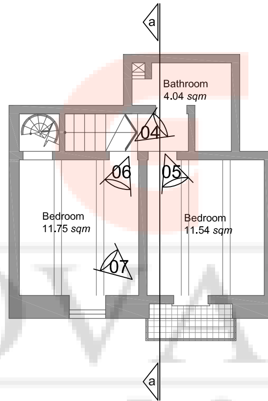
First Floor level existing Scale 1:100
