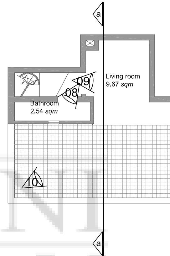
Recessed Floor level existing Scale 1:100
