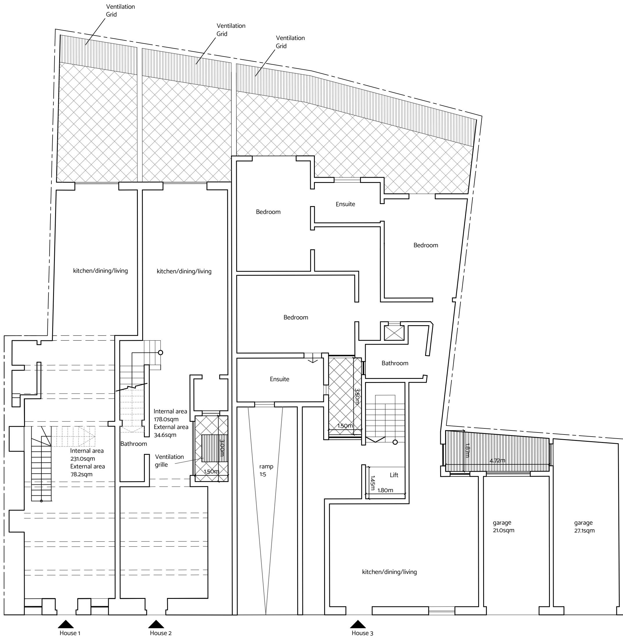
Proposed Ground Floor Level Plan Scale 1:100 clean copy
