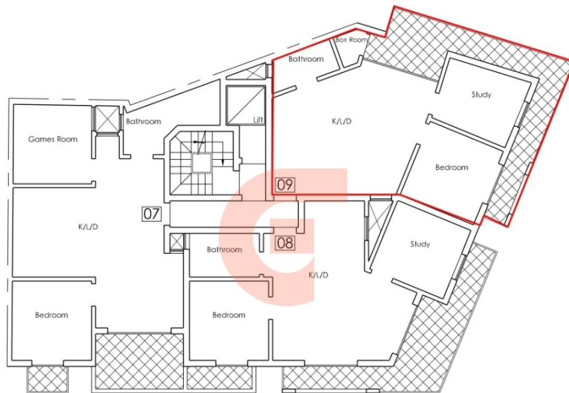
As Proposed Third Floor
