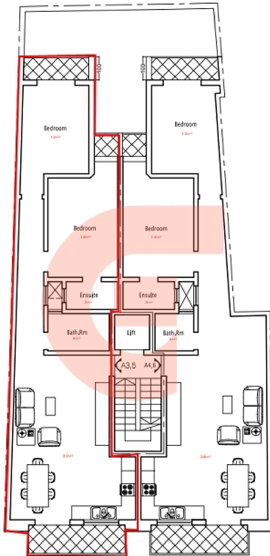
○ 2nd Floor Plan Scale 1:100
